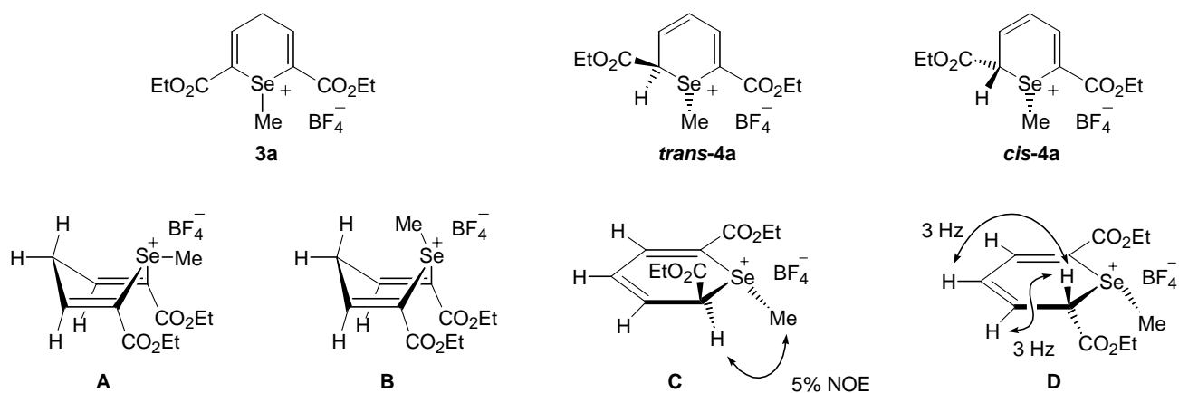
Figure 1 Stereoisomers for 4 H - and 2 H -selenopyranium salts
