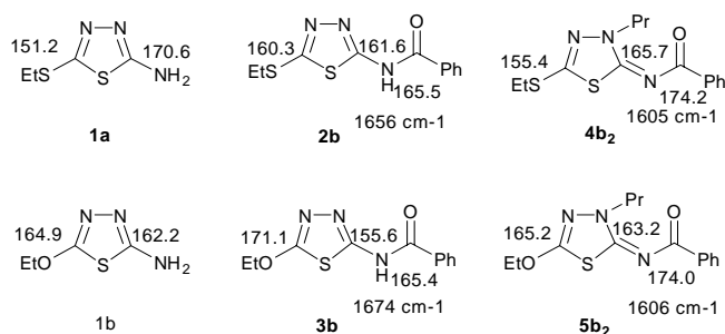
Scheme 2. \delta_{\text{H}} (300 MHz; DMSO- d_6 ; Me _4 Si), \nu (KBr pellet).
