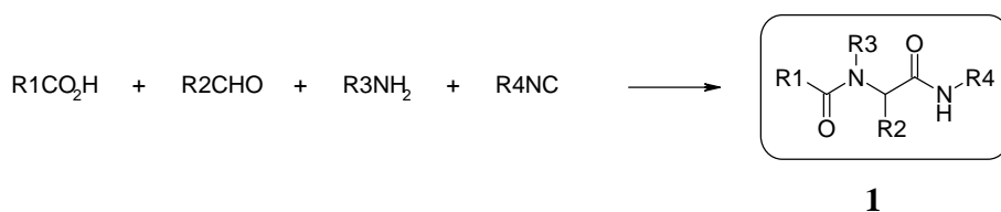
Scheme 1. Ugi reaction
