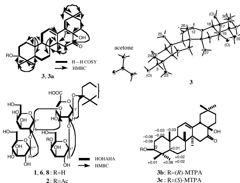
Figure 1. HMBC Correlations, X-Ray Crystallographic analysis, and Modified Mosher's Method
