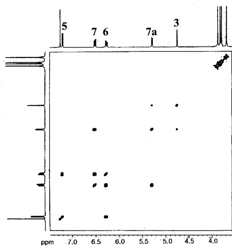
Figure 1. ^1\text{H} - ^1\text{H} COSY spectrum of 4.
