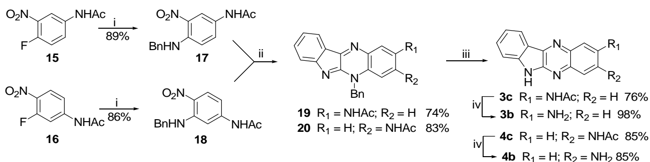
Scheme 4 Reagents and conditions: i, \text{BnNH}_2 , \text{AcONa} , \text{EtOH} , reflux; ii, \text{H}_2 , Raney Ni, \text{EtOH} then 1 , \text{AcOH} , reflux; iii, \text{H}_2 , Pd-C, \text{EtOH} ; iv, \text{HCl} , \text{EtOH} , reflux.
