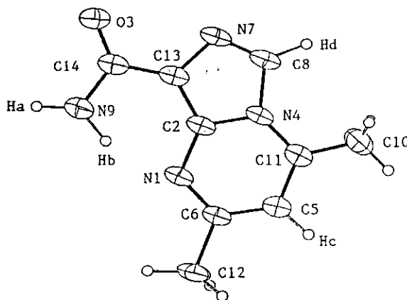
Figure 1. Perspective view and atom labelling of the X-ray structure of compound ( 7a ).
