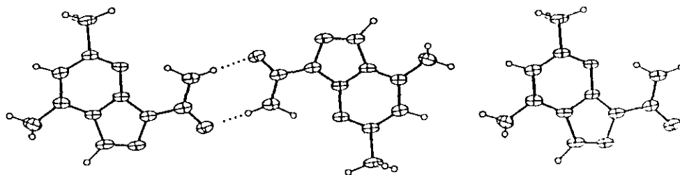
Figure 2. An ORTEP drawing shows the intermolecular H-Bond within dimer (left) and the hydrophobic interactions between dimers which maintain the extension along 2B \pm A directions.
