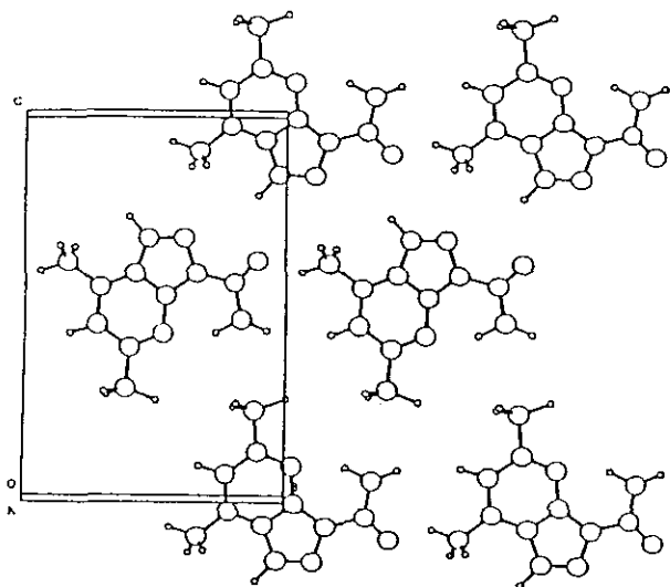
Figure 3A (left). The hydrophobic interactions between interlaced.
