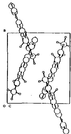
Figure 3B (right). A perspective drawing shows intermolecular stacking.
