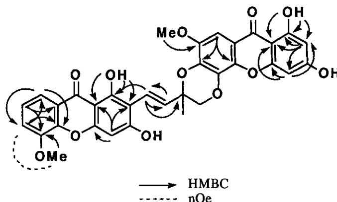
Figure 3 HMBC ( J = 10 Hz) and nOe results in 2
