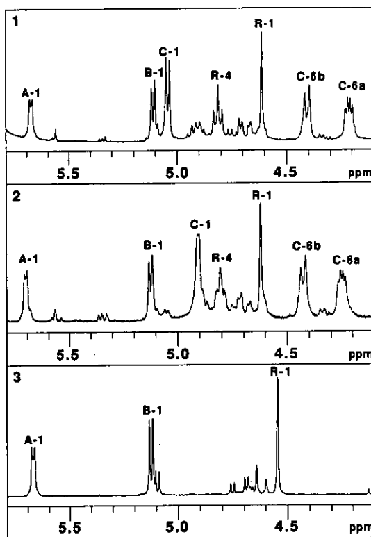
Figure 2 ^1\text{H} -NMR spectra of the sugar regions of pigment 1 (upper, 1), pigment 2 (middle, 2), and deacyl pigment 1 and 2 (lower, 3) at 500 MHz in \text{DCI/DMSO}-d_6 (1:9).
