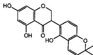
licoisoflanone (4)
