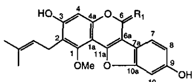
R 1 =O glycyrol (5) R 1 =H 2 glyrallin A (6)
