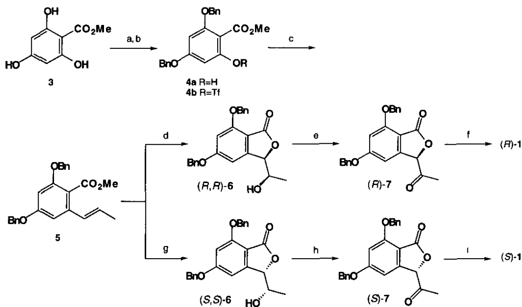
Scheme 1. a) BnBr (2.1 eq.), K 2 CO 3 , NaI, DMF, rt, 12 h, 47%. b) Tf 2 O, pyridine, CH 2 Cl 2 , -40 °C, 0.5 h; 0 °C, 3.5 h, 77%. c) MeCH=CHSnBu 3 ( EZ mixture, 1.7 eq.), Pd(0)[PPh 3 ] 4 , LiCl, THF, 90 °C, 7 d; recryst'n, 59%. d) AD-mix-β, MeSO 2 NH 2 , Bu'OH, H 2 O, 4 °C, 12 d, recryst'n, 75%. e) Dess-Martin reagent, CH 2 Cl 2 , rt, 1 h, 91%. f) H 2 , 10% Pd(OH) 2 -C, AcOEt, rt, 15 min, 71%. g) AD-mix-α, MeSO 2 NH 2 , Bu'OH, H 2 O, 4 °C, 3 d; recryst'n, 79%. h) Dess-Martin reagent, CH 2 Cl 2 , rt, 1 h, 99.5%. i) H 2 , 10% Pd(OH) 2 -C, AcOEt, rt, 15 min, 87%.
