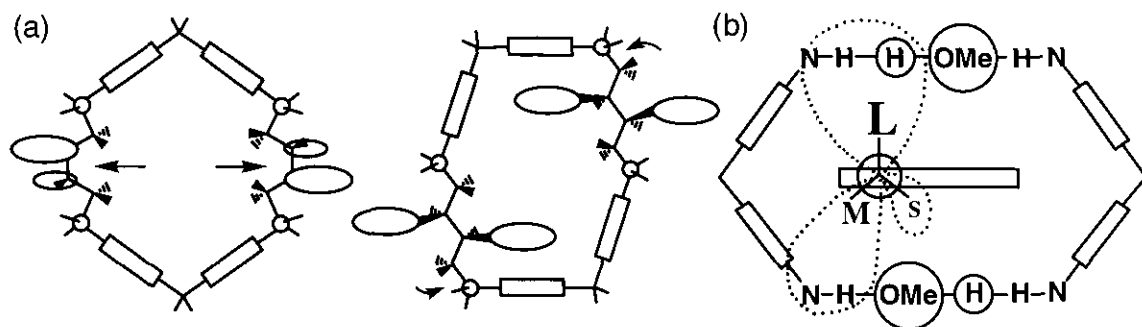
Figure 5. (a) Possible structures of the inclusion cavities of tetraprotonated TCP44 ( 1 \cdot 4H^+ ). Hexagonal cavity with the C-C gauche conformation (left) and rectangular cavity with the C-N gauche conformation (right). In each figure, rectangles, ellipses and circles indicate benzene rings, methoxy groups and ammonium (protonated amine) nitrogens, respectively. Arrows exhibit the gauche bonds. (b) A possible model of chiral recognition by protonated TCP44 ( 1 ) in acidic media. Three open spaces, L (large), M (medium) and S (small), of the chiral cavity can accommodate the three substituents attached to the chiral center of the complexed aromatic guest.
