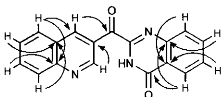
Figure 2 Significant HMBC correlations ( J_{\text{CCH}} = 8 Hz) of 2
