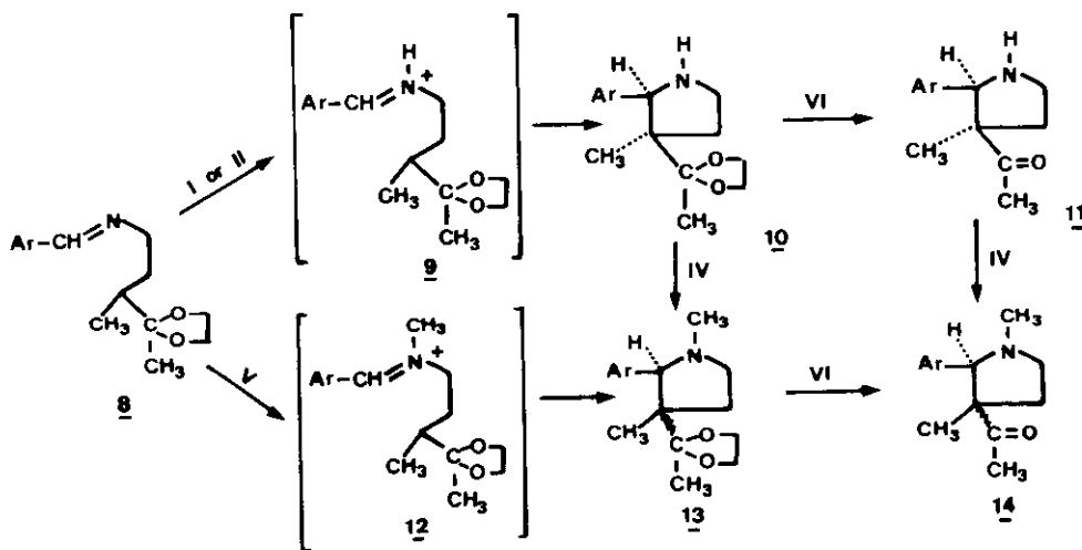
SCHEME III
