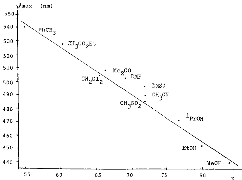
Figure. Solvent effect on uv. spectrum of 1-(p-toluoyl-cyanomethyl)-2,4,6-triphenylpyridinium ylid (10a).
