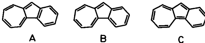
Fig. 5. Kekulé structures belonging to 2,3-benzazulene
