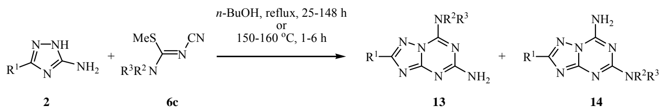
Scheme 5
