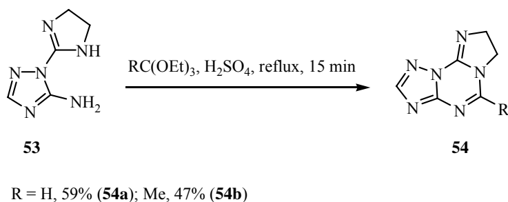
Scheme 23
