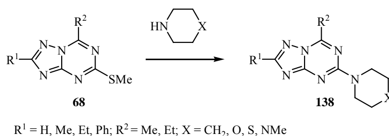
Scheme 58
