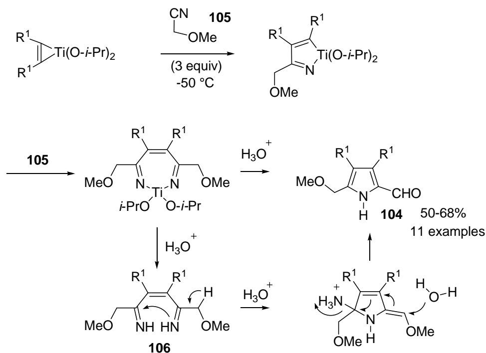
Scheme 49
