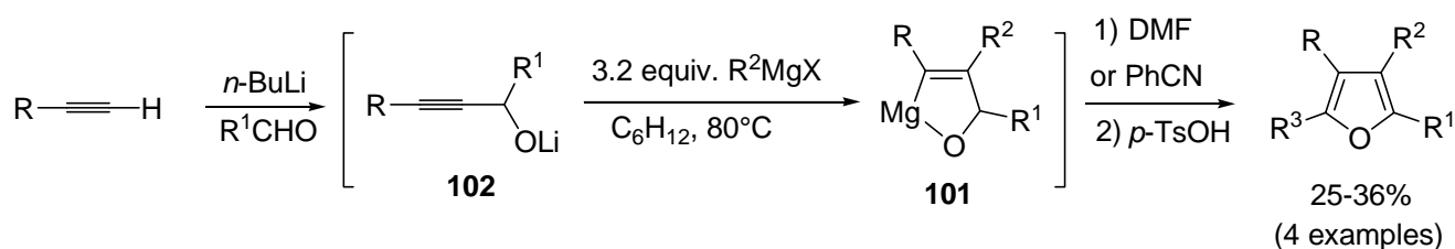
Scheme 46
