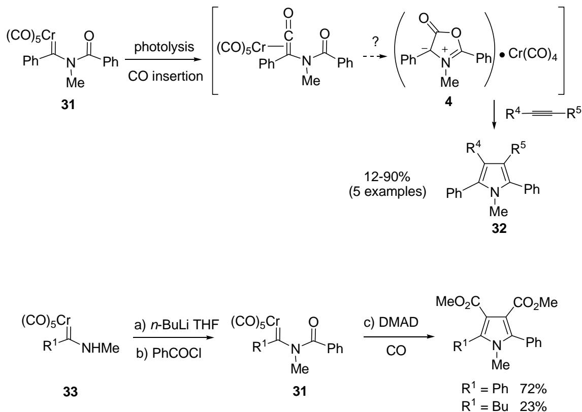
Scheme 9
