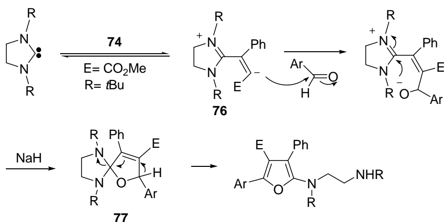
Scheme 27
