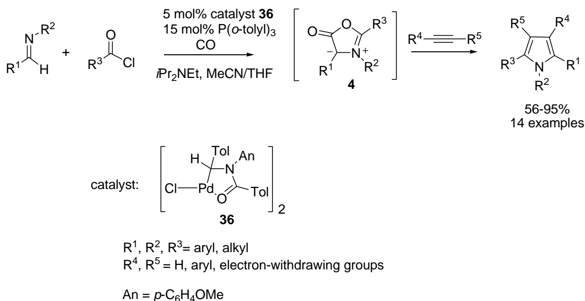
Scheme 11
