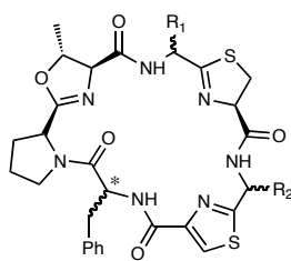
27: (R)-CH(Me)Et, (R)-Me, S 28: (R)-CH(Me)Et, (S)-Me, S 29: (S)-CHMe 2 , (R)-CH 2 -Phe, S 31: (R)-CHMe 2 , (R)-CH 2 -Phe, S 33: (R * )-CHMe 2 , (R * )-CH 2 -Phe, S 34: (S)-CH(Me)Et, (R)-CHMe 2 , R
