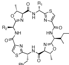
38: R 1 = Me, R 2 = CH 2 CHMe 2 39: R 1 = Me, R 2 = CHMe 2 40: R 1 = Me, R 2 = CH(Me)Et 41: R 1 = CHMe 2 , R 2 = CHMe 2
