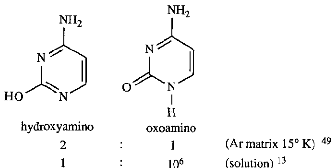
Scheme 21. Relative Abundance of Cytosine Tautomers in Different Media
