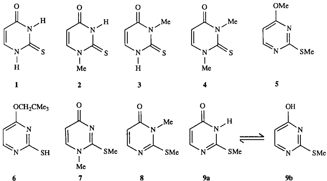
Scheme 20. Predominant Gas Phase Tautomers for Monothioracils
