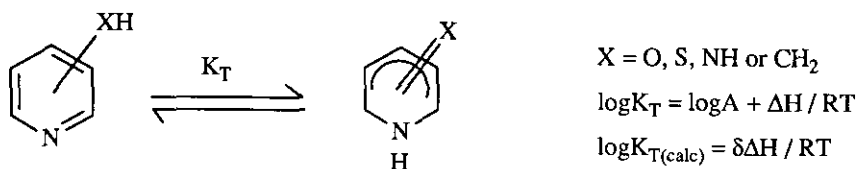
Scheme 22. Tautomeric Equilibria in Substituted Pyridines
