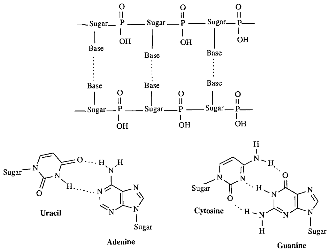
Scheme 8. Tautomerism in the Nucleic Acids
