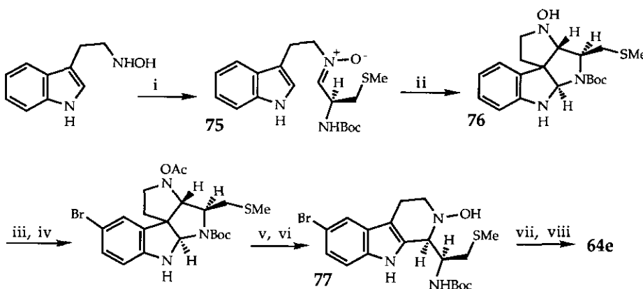
Scheme 27 Reagents : i, (S)-MeSCH 2 CH(NHBoc)CHO, CH 2 Cl 2 , room temperature, 2 h (96%); ii, TFA, room temperature (69%); iii, Ac 2 O; iv, NBS, room temperature, 20 min; v, deacetylation (75% overall iii-v); vi, 3xTFA, room temperature, 40 h (33%); vii, NCS, CH 2 Cl 2 , -78°C, 2 h (4%); viii, deprotection (76%).
