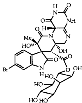
surugatoxin 88
