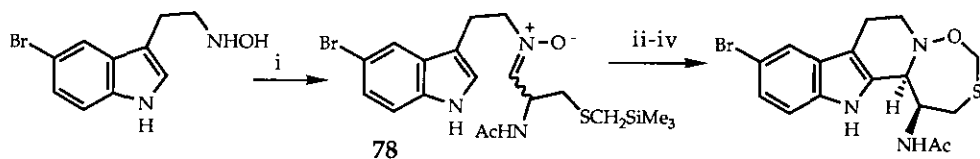
Scheme 28 Reagents : i, Me 3 SiCH 2 SCH 2 CH(NHAc)CHO, MgSO 4 , 7 h (28%); ii, TFA, CH 2 Cl 2 , room temperature, 16 h (24%); iii, MCPBA, NaHCO 3 (70%); iv, 23→80°C (17-21%).
