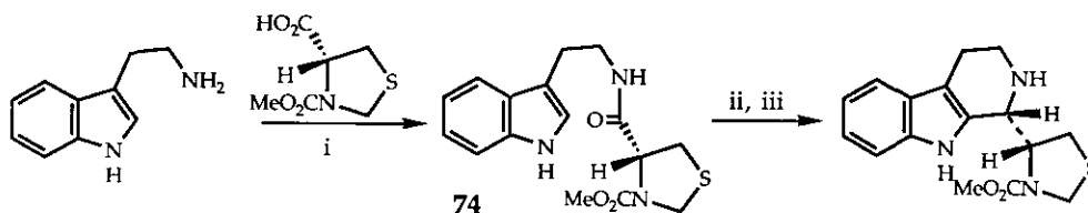
Scheme 26 Reagents : i, DCC, CH 2 Cl 2 (98%); ii, POCl 3 , PhH, reflux; iii, NaBH 4 (63% overall ii, iii, plus diastereoisomer (20%)).
