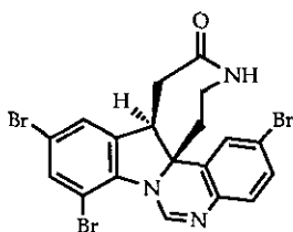
hinckdentine 87
