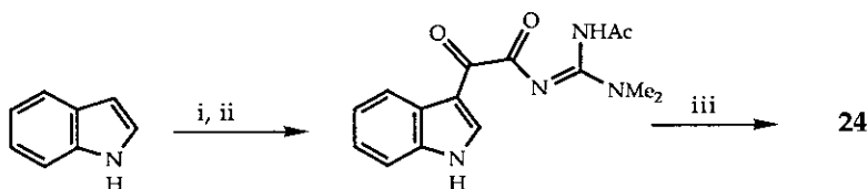
Scheme 5 Reagents : i, (COCl) 2 ; ii, AcHNC(=NH)NMe 2 ; iii, H 2 O (no yields given).
