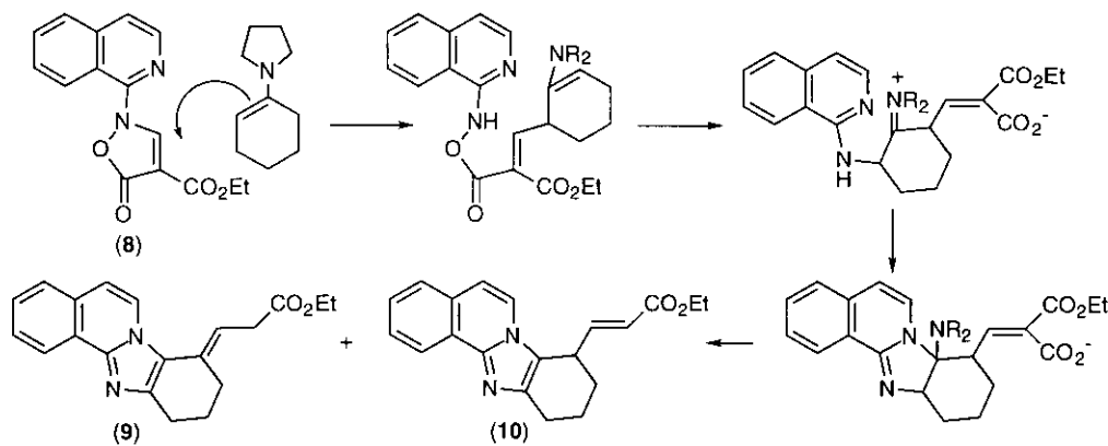
Scheme 9
