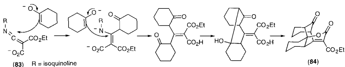
Scheme 30
