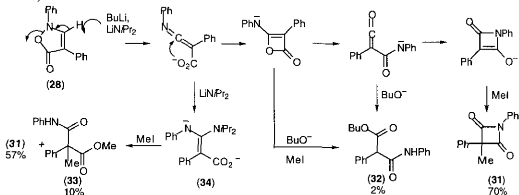
Scheme 18
