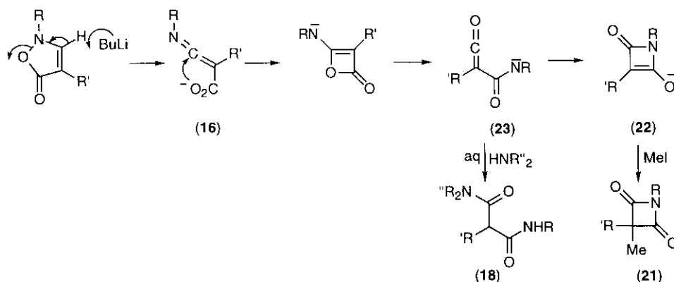
Scheme 15
