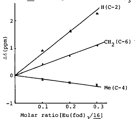
Fig. 2 Induced Signal Shifts of PMR spectra of 16 in the presence of \text{Eu}(\text{fod})_3
