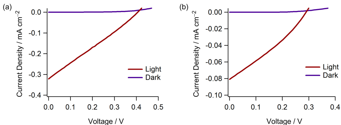
Figure 4. Photovoltaic performance of BJJ solar cells: (a) cell 1 and (b) cell 2
