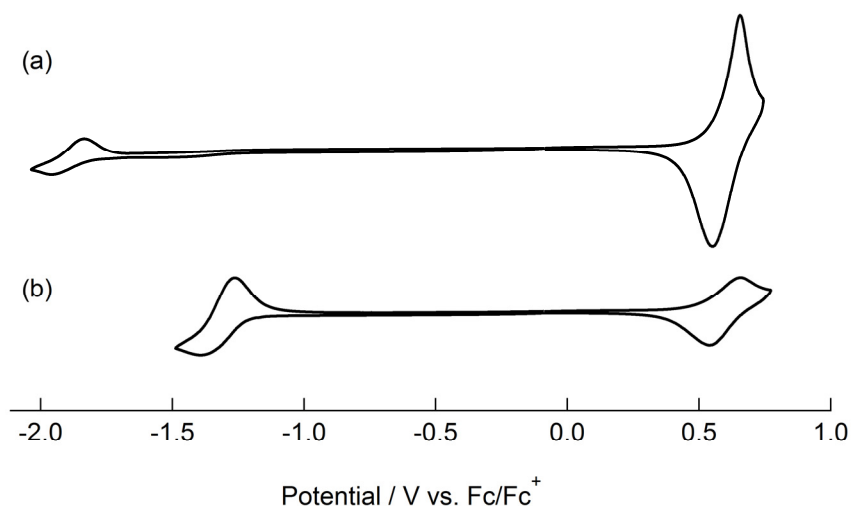
Figure 2. Cyclic voltammograms of polymer films; (a) 1 and (b) 2
