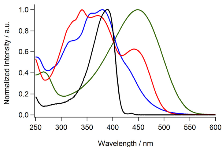
Figure 1. UV-vis absorption spectra of polymers in dichloromethane; —: 1 , —: 2 , —: PFO, —: P3HT
