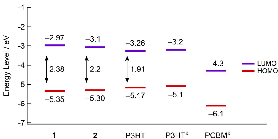
Figure 3. HOMO/LUMO energy diagram of polymers ( 1 ) and ( 2 ) with P3HT and PCBM ( a Ref. 3a); values given in eV
