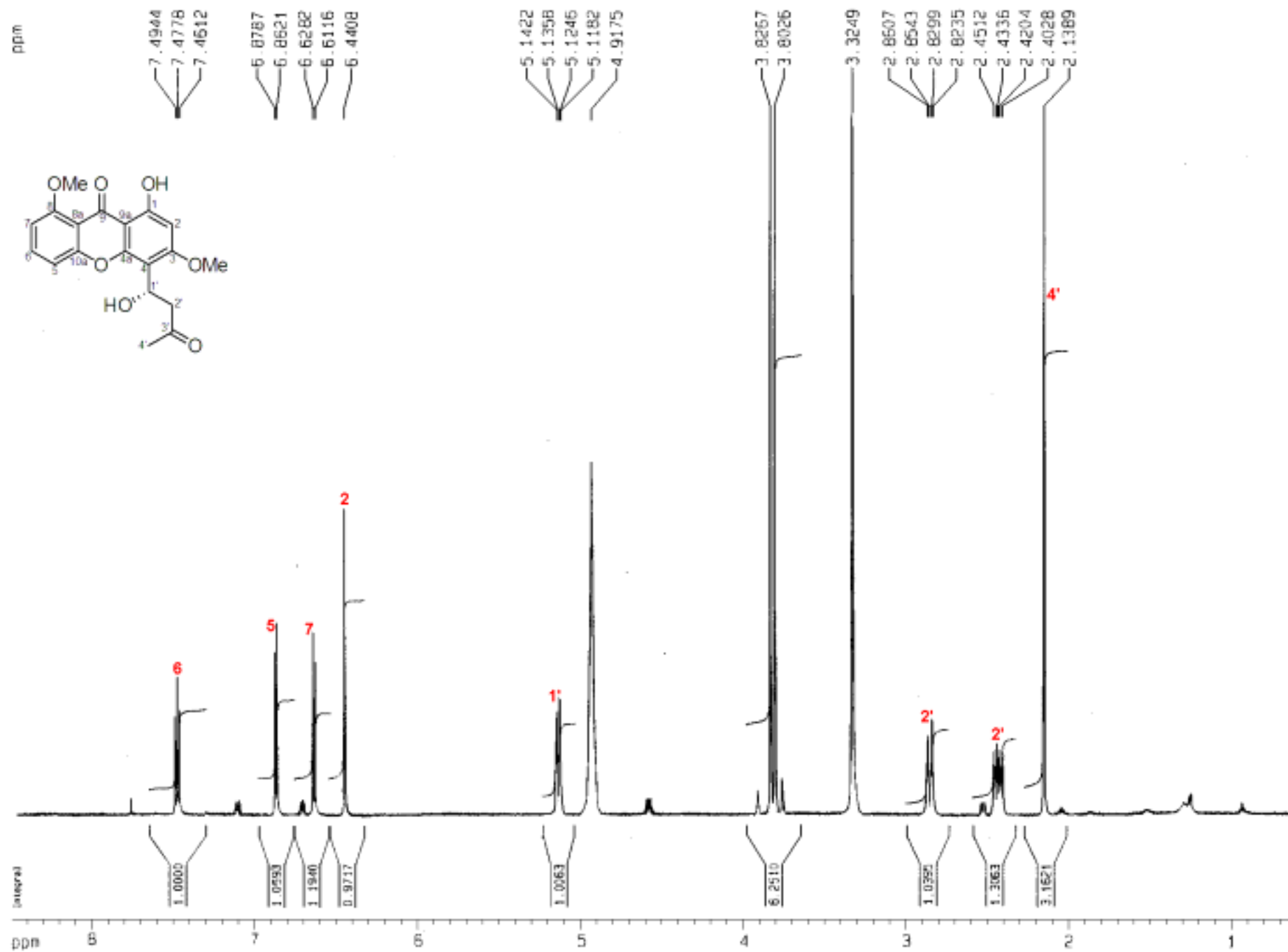
Figure S4. ^1\text{H} NMR spectrum of ( S )-1-hydroxy-4-(1-hydroxy-3-oxobutyl)-3,8-dimethoxy-9 H -xanthen-9-one ( 2 )
