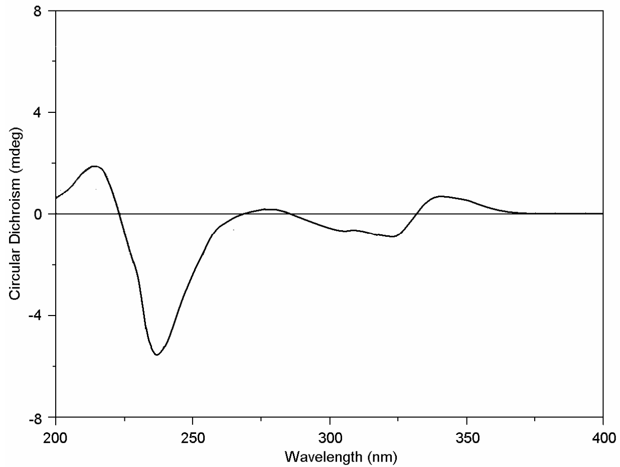
Figure S5. CD spectrum of ( S )-1-hydroxy-4-(1-hydroxy-3-oxobutyl)-3,8-dimethoxy-9 H -xanthen-9-one (2)
