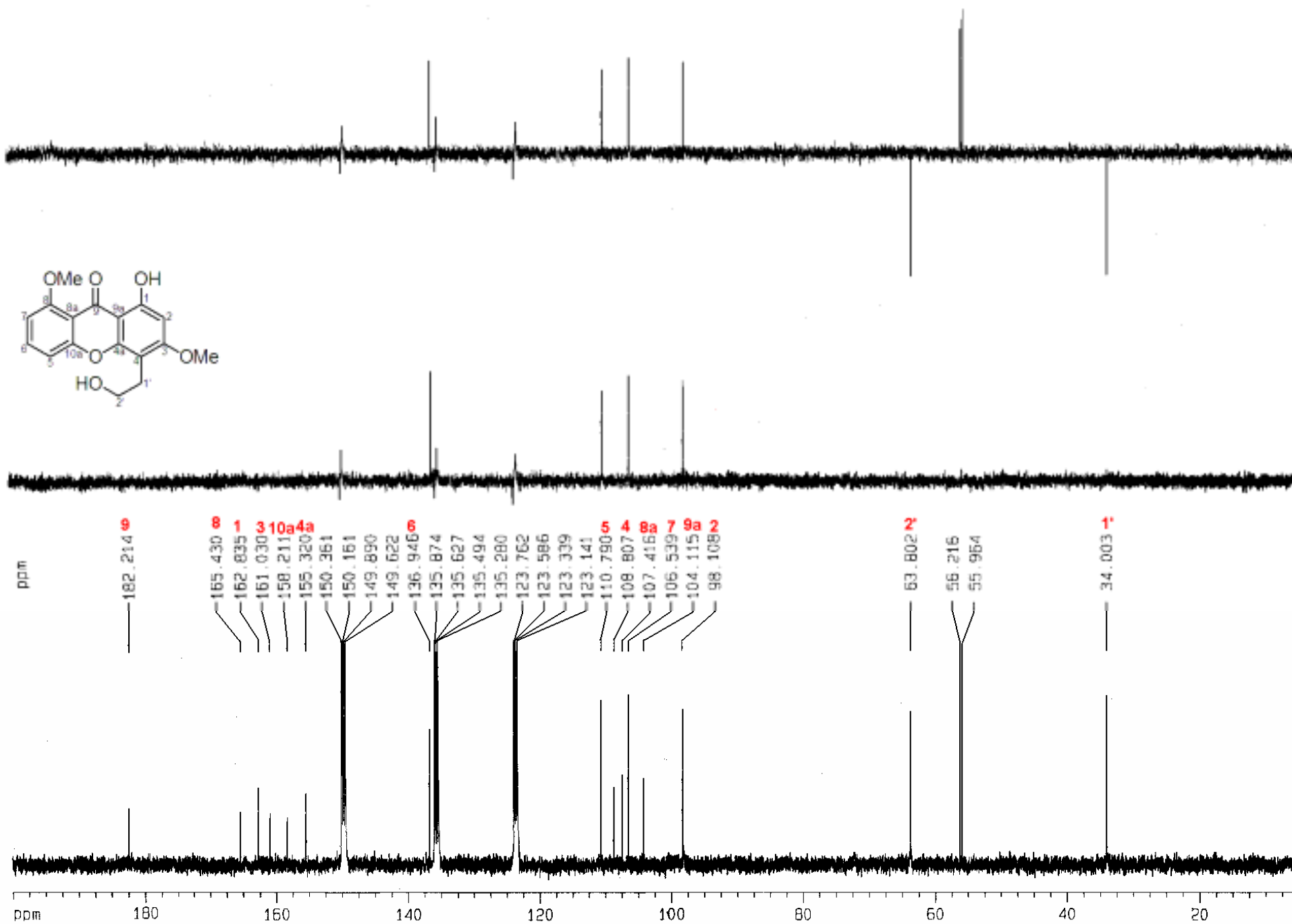
Figure S1. ^{13}\text{C} NMR and DEPT spectrum of 1-hydroxy-4-(2-hydroxyethyl)-3,8-dimethoxy-9 H -xanthen-9-one ( 1 )
