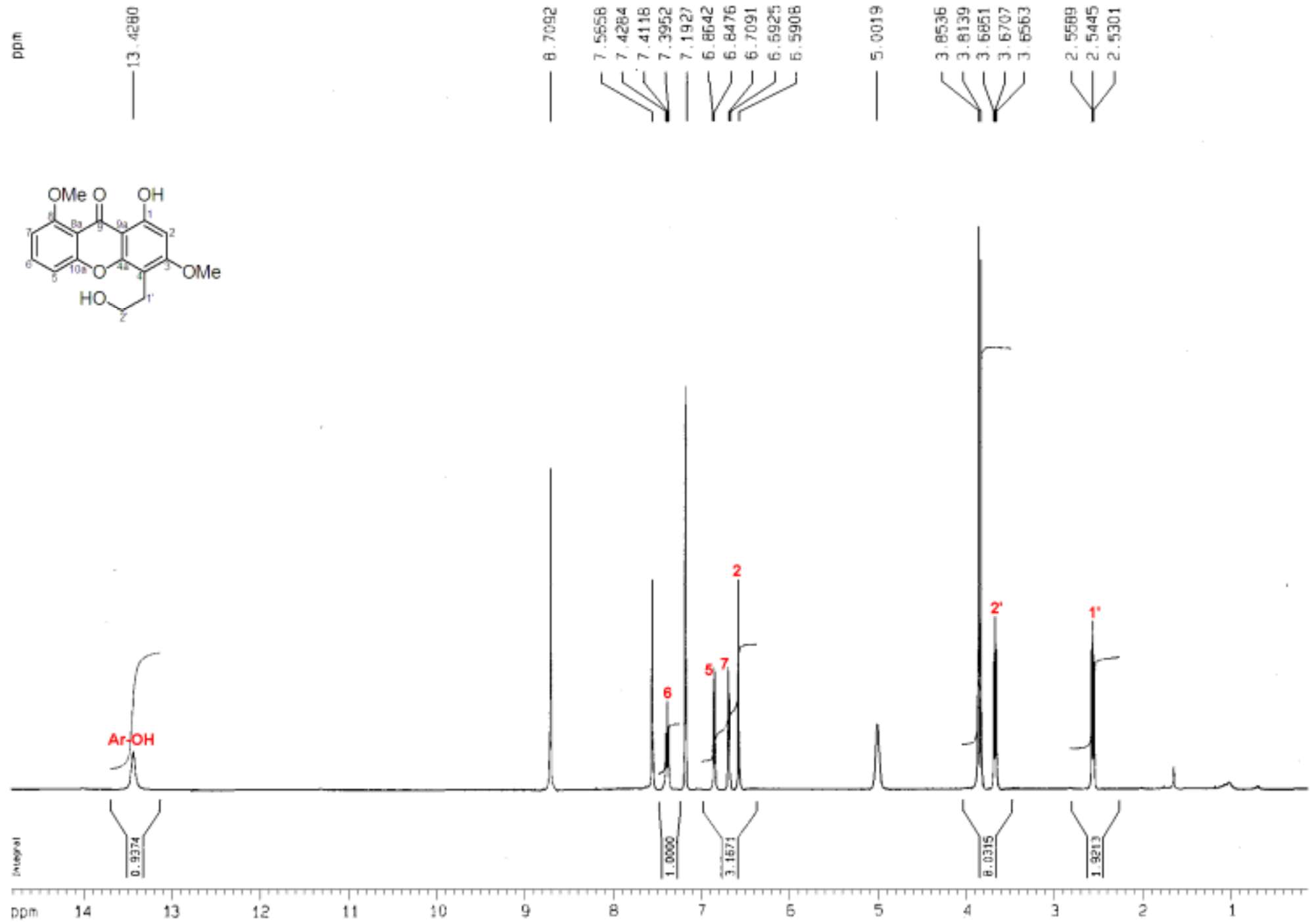
Figure S2. 1 H NMR spectrum of 1-hydroxy-4-(2-hydroxyethyl)-3,8-dimethoxy-9H-xanthen-9-one (1)
