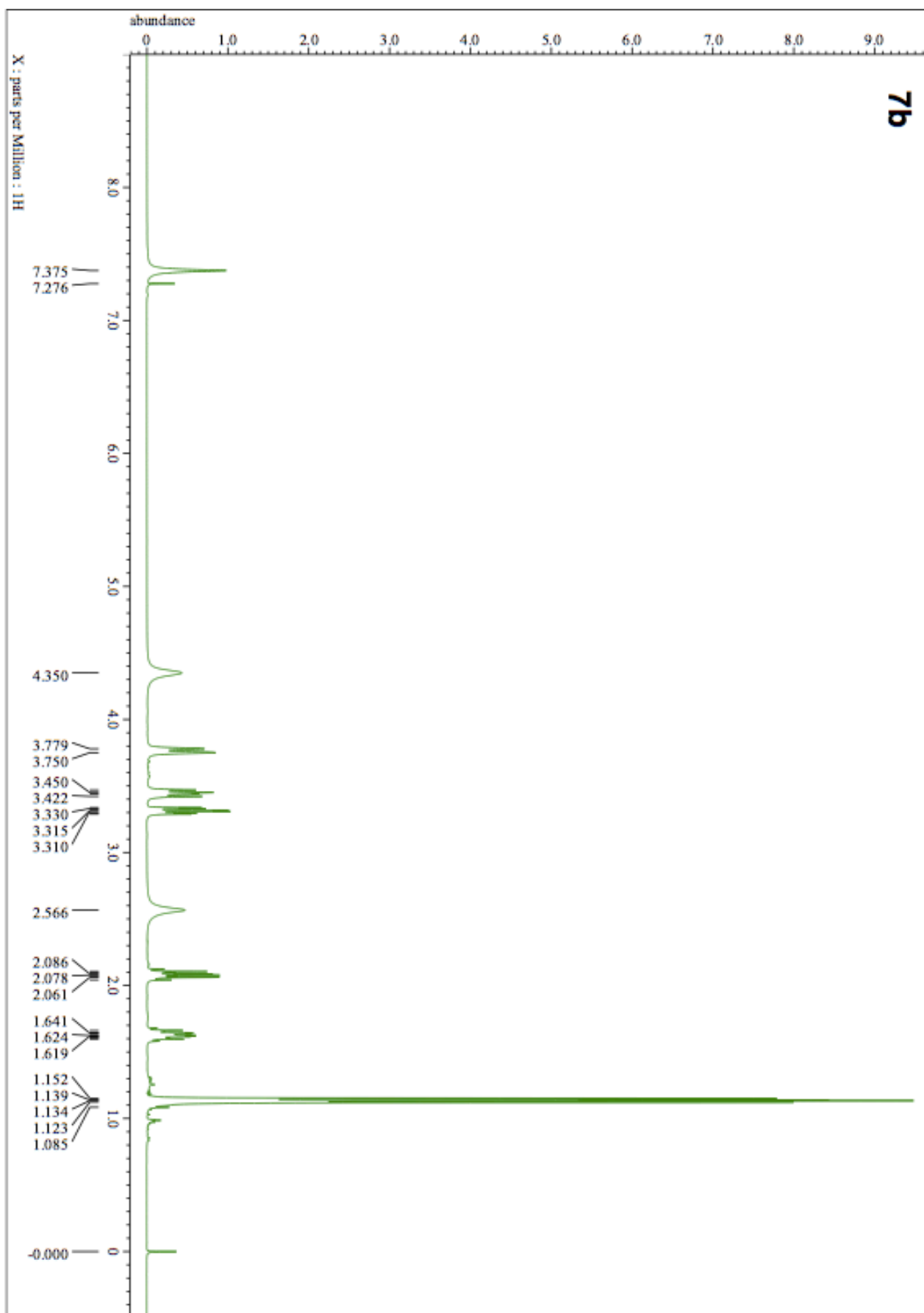
Supplementary Figure S17. ^1\text{H} NMR spectrum of 7b .
