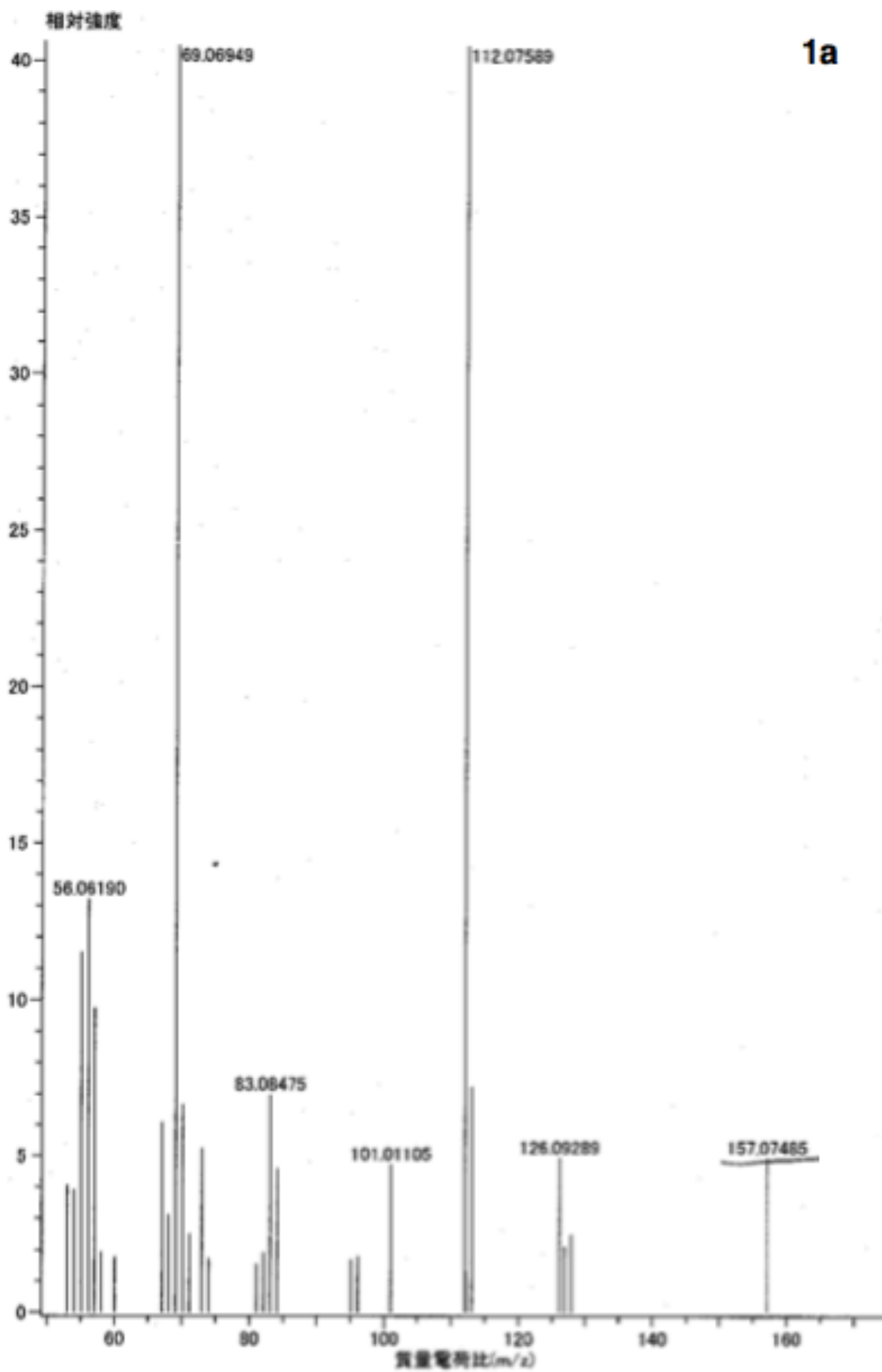
Supplementary Figure S4. MS spectrum of 1a.
