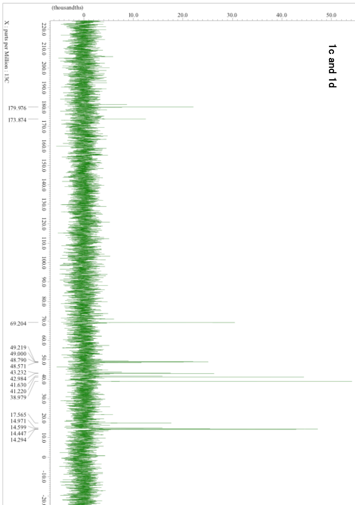
Supplementary Figure S10. ^{13}\text{C} NMR spectrum of mixture of 1c and 1d .
