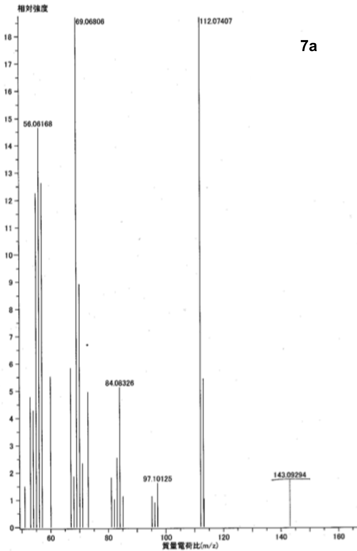
Supplementary Figure S16. MS spectrum of 7a.
