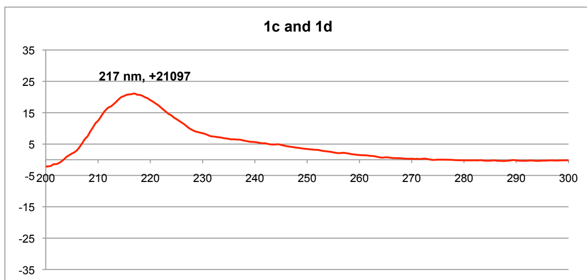
Supplementary Figure S25. CD spectra of 1a , 1b , and mixture of 1c and 1d .
