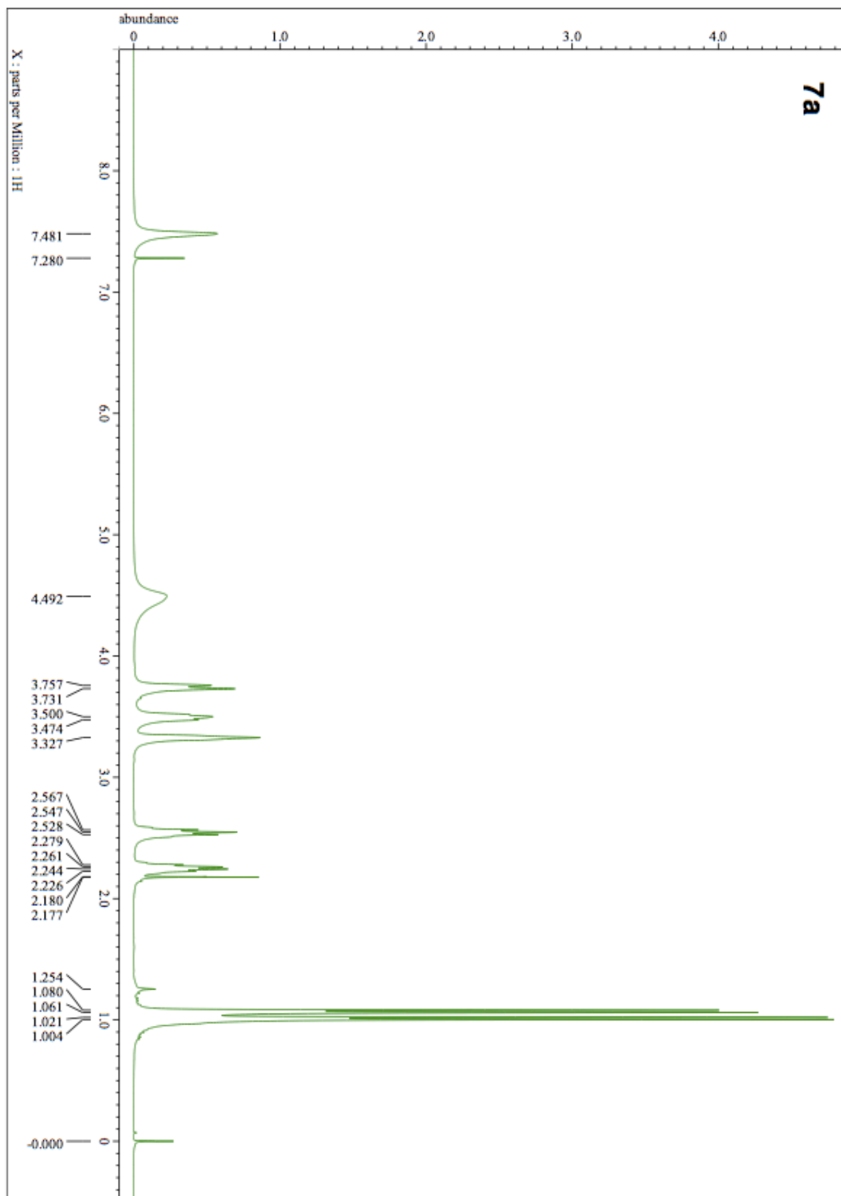
Supplementary Figure S13. ^1\text{H} NMR spectrum of 7a .
