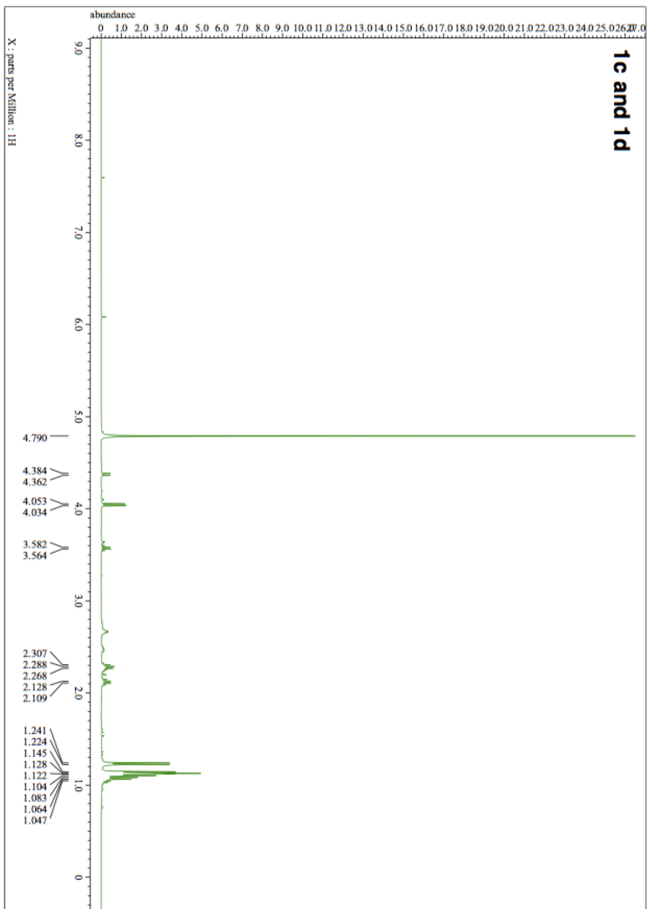
Supplementary Figure S9. ^1\text{H} NMR spectrum of mixture of 1c and 1d .
