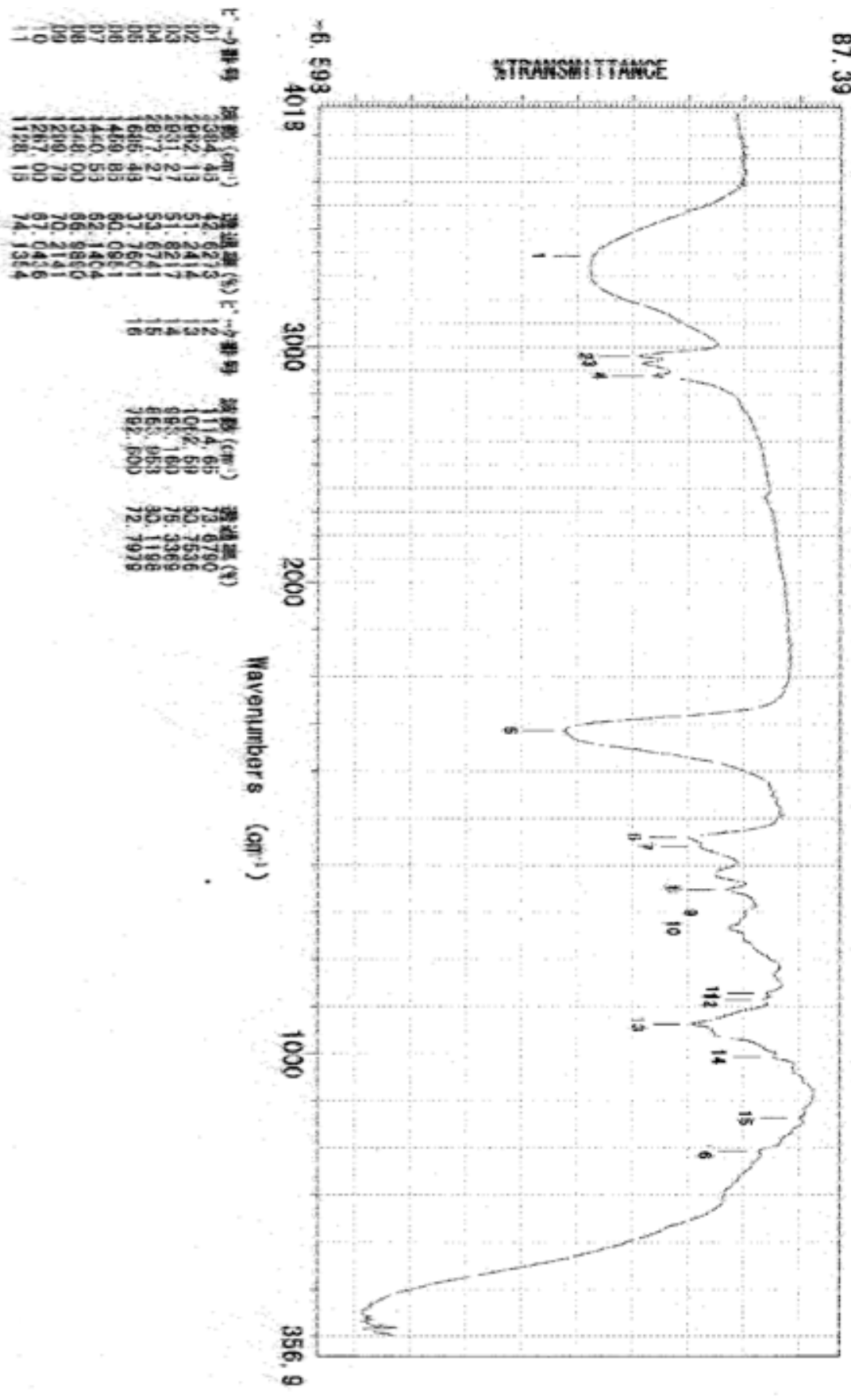
Supplementary Figure S23. IR spectrum of mixture of 7c and 7d.
