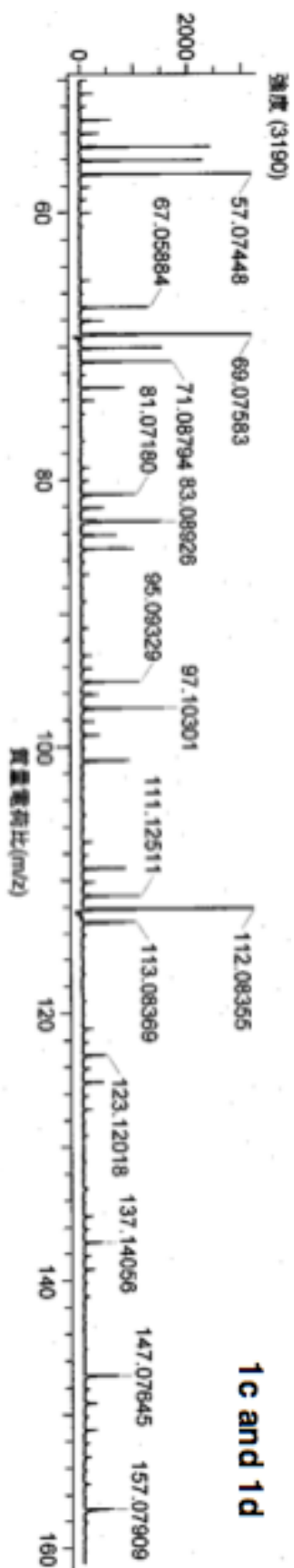
Supplementary Figure S12. MS spectrum of mixture of 1c and 1d .
