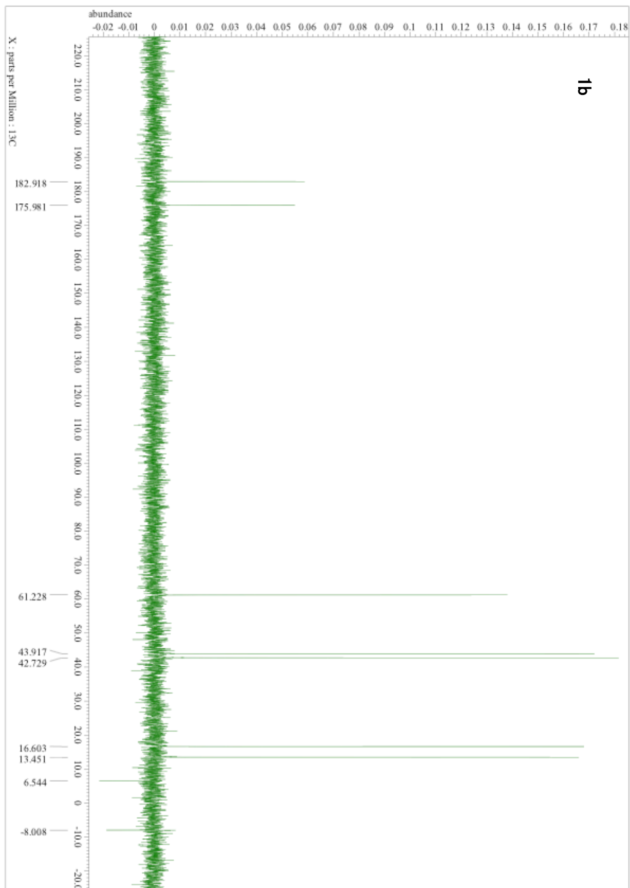
Supplementary Figure S6. ^{13}\text{C} NMR spectrum of 1b .
