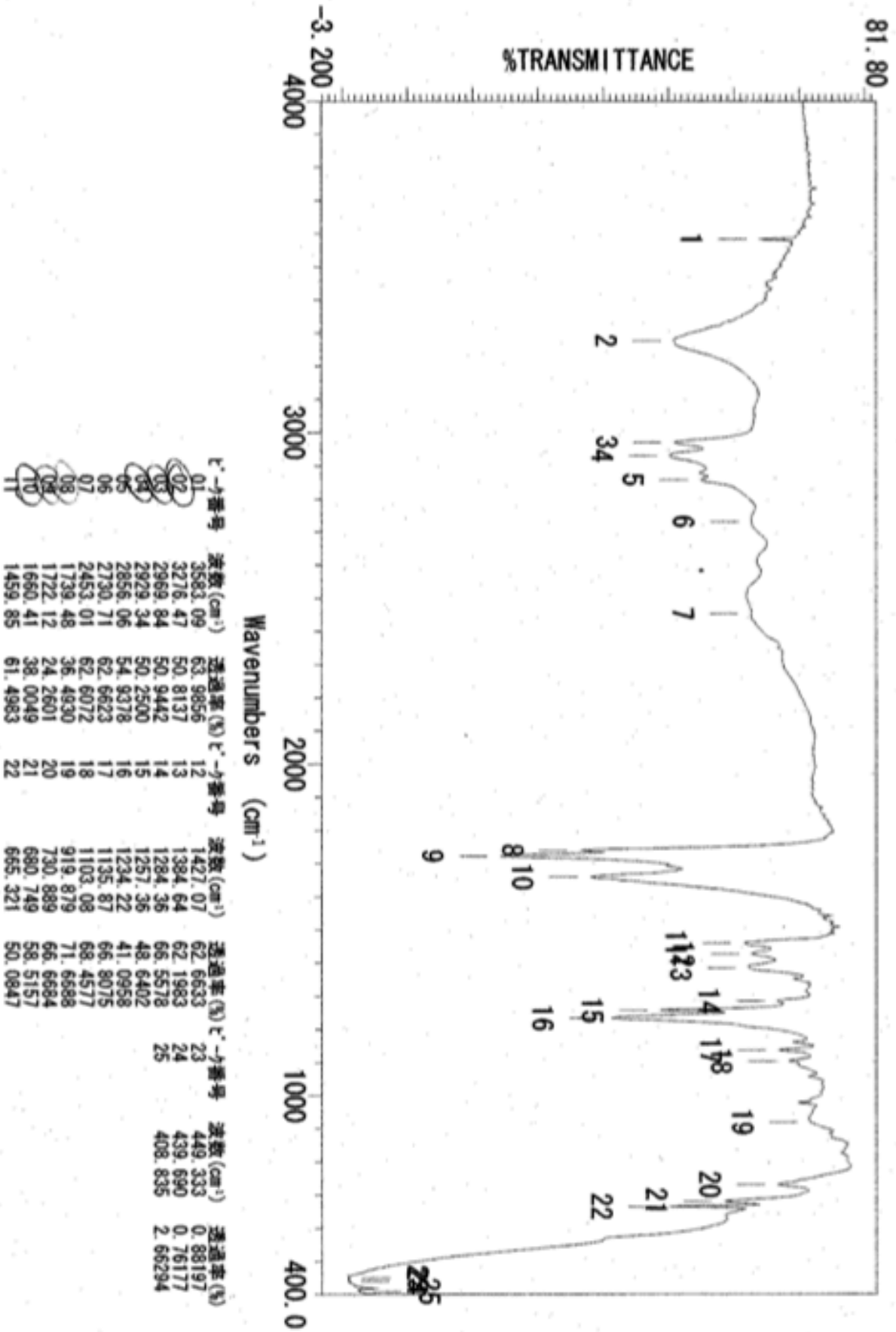
Supplementary Figure S7. IR spectrum of 1b.
