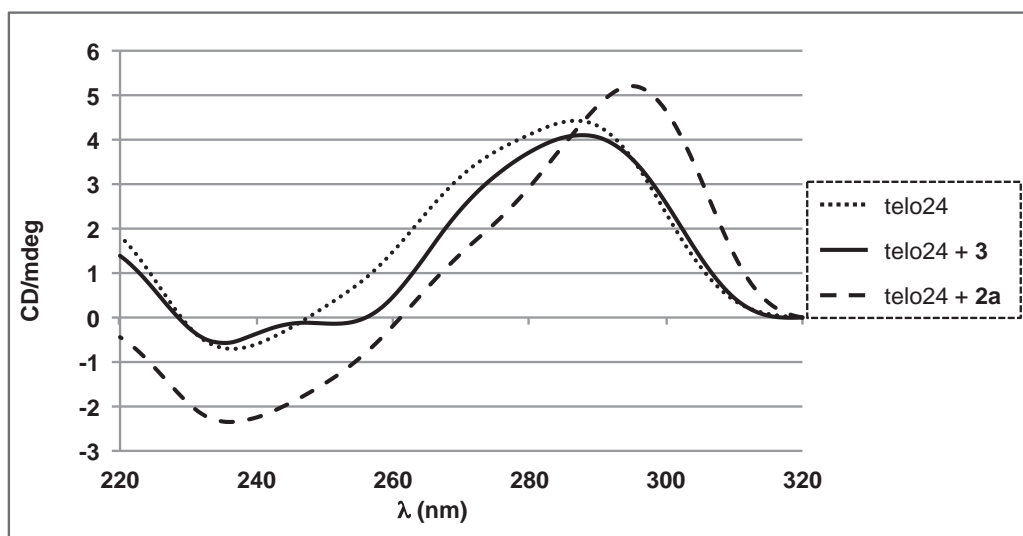
Figure S1. CD spectra of a telo24 (d[TTAGGG] 4 ) in the absence or presence of 3 and 2a (five equivalent to DNA). These spectra were measured in the presence of 100 mM potassium chloride conditions.
