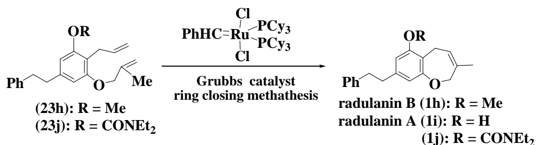
Scheme 7. Ring-closing Metathesis
