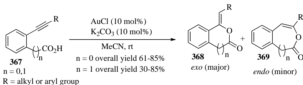
Scheme 109. Au(I)-Catalyzed intramolecular cyclization of \gamma - and \delta -alkynes acids to alkylidene lactones
