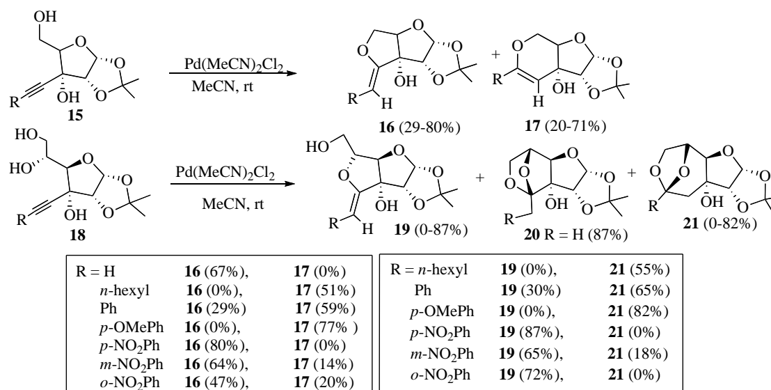
Scheme 6. Pd-Catalyzed 5- exo vs 6- endo -dig cyclization
