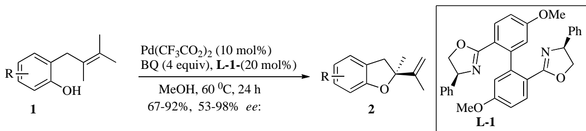
Scheme 2. Pd-Catalyzed enantioselective synthesis of benzofurans
