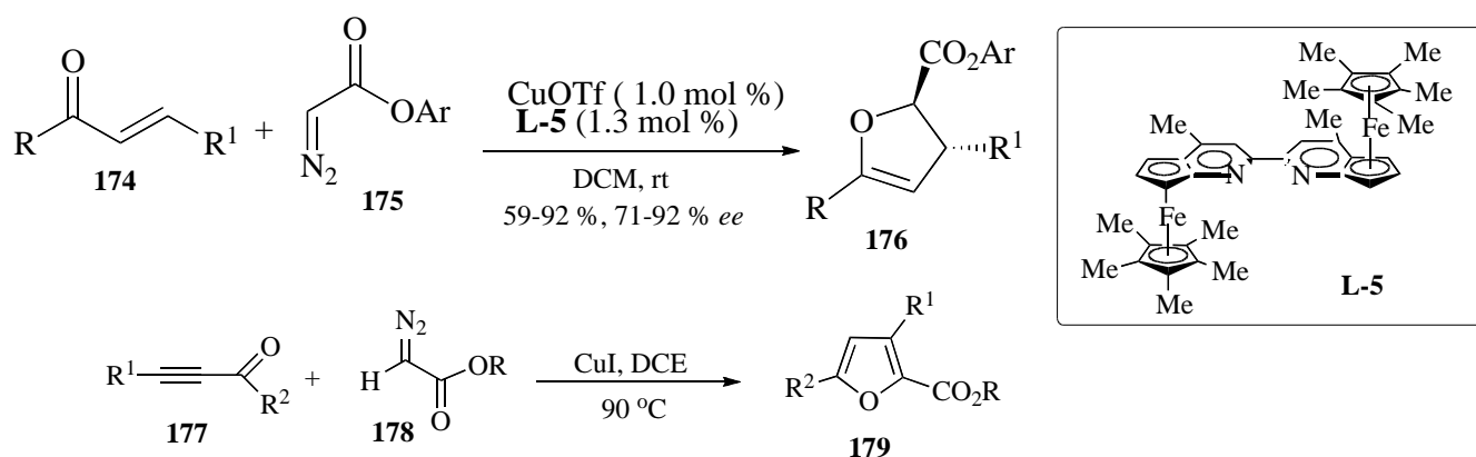
Scheme 55. Cu-Catalyzed stereoselective synthesis of 2,3-dihydrofurans from enones and diazo compounds
