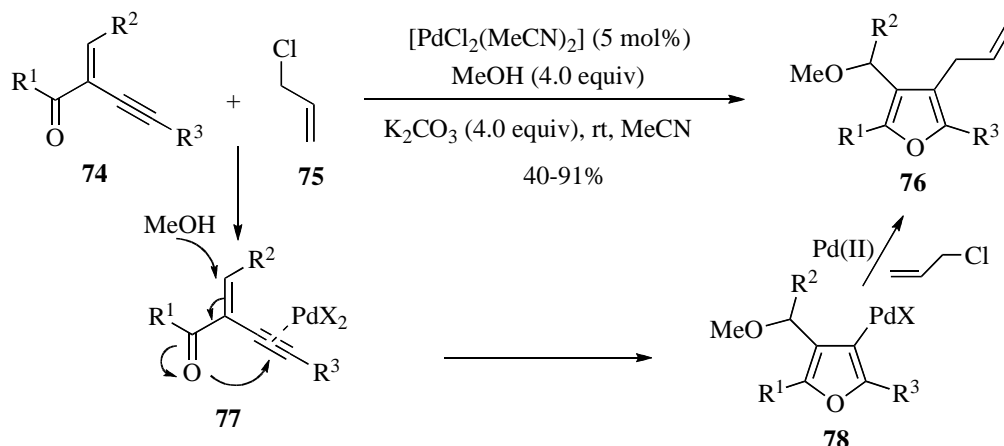
Scheme 25. Pd-Catalyzed synthesis of tetrasubstituted furans
