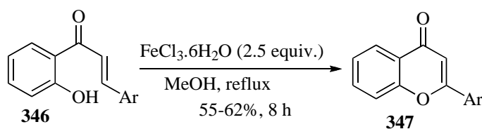
Scheme 102. Fe(III)-Catalyzed synthesis of flavones from 2'-hydroxychalcone
