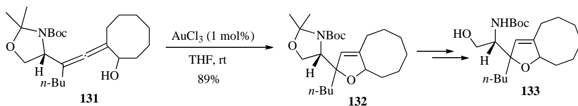
Scheme 42. Au-Catalyzed synthesis of bicyclic furanomycin derivative
