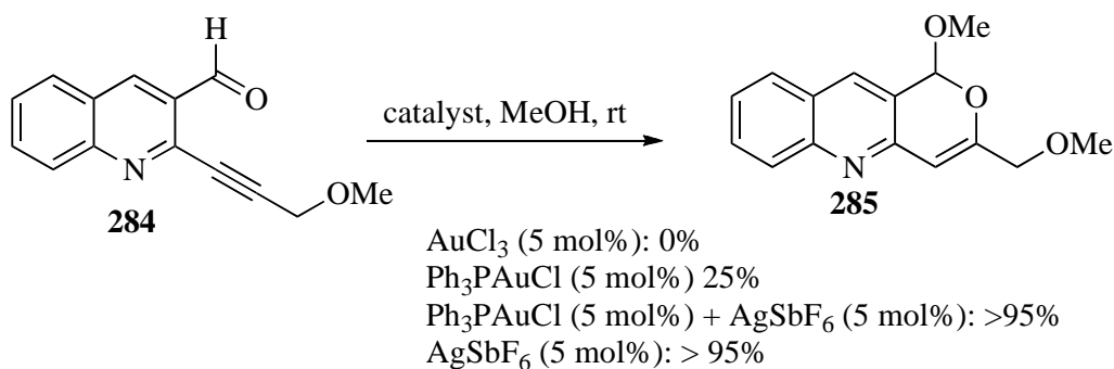
Scheme 86. Au-Catalyzed reaction of 1-alkynyl-2-carbonyl-quinolines to pyranoquinolines
