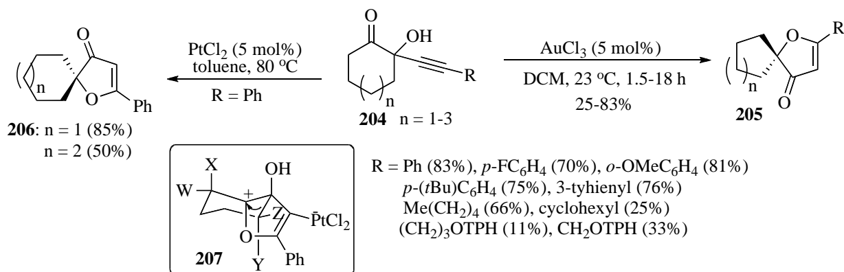
Scheme 65. Cycloisomerization of alkyneones having a hydroxyl group at the \alpha -position to furanones
