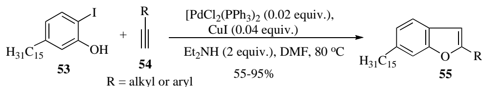
Scheme 17. Pd-Catalyzed synthesis of substituted benzofurans
