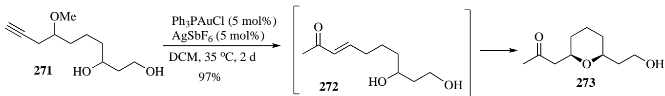
Scheme 82. Au-Catalyzed synthesis of 2,6- cis -tetrahydropyrans
