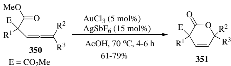
Scheme 104. Au(III)-catalyzed cyclization of allene-substituted malonates to \beta,\gamma -unsaturated \delta -lactones
