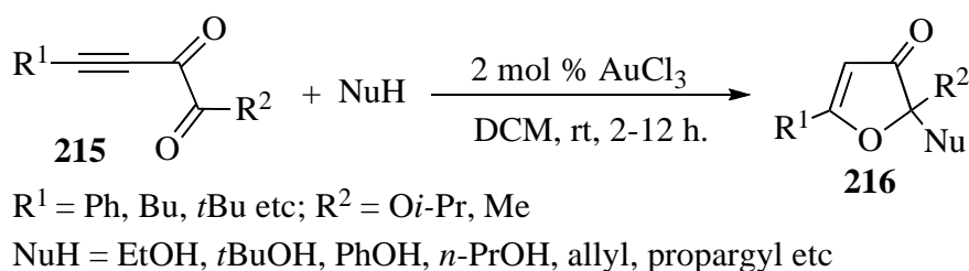
Scheme 68. Au-Catalyzed synthesis of substituted 3(2 H )-furanones
