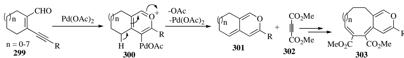
Scheme 90. Pd(OAc) 2 -Catalyzed synthesis of pyran derivatives fused with medium to large rings
