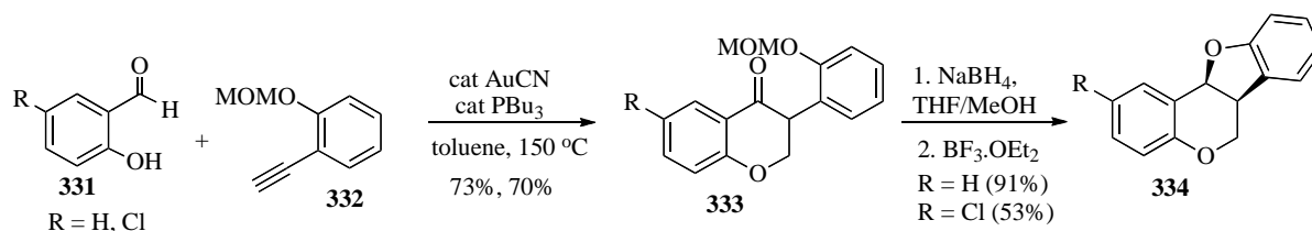
Scheme 99. Au(I)-Catalyzed synthesis of (±)-pterocarpan
