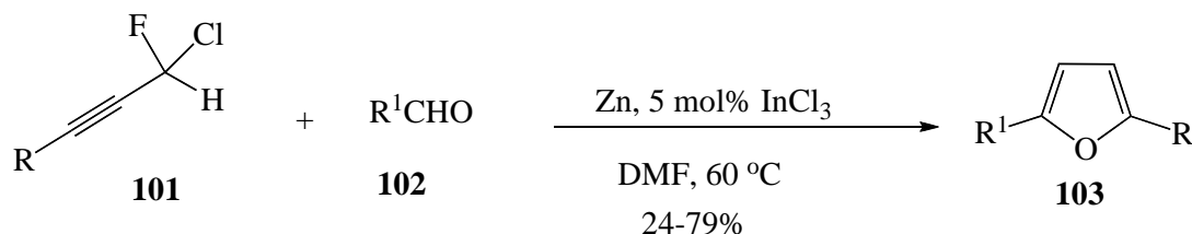
Scheme 32. InCl 3 -Catalyzed synthesis of 2,5-disubstituted furans from fluoropropargyl chloride
