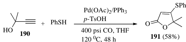
Scheme 59. Pd-catalyzed synthesis of 4-thiophenylfuranones
