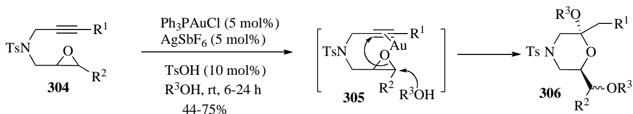
Scheme 91. Au(I)-Catalyzed ring-opening of epoxides to 2,6- trans -substituted morpholine
