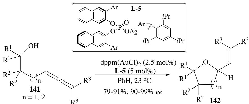
Scheme 46. Au(I)-Catalyzed enantioselective hydroxylation of terminal disubstituted allenes
