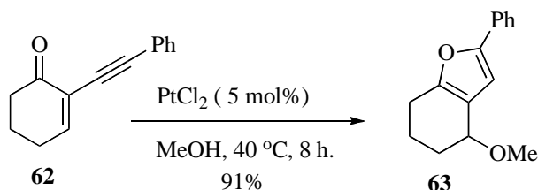
Scheme 20. Pt-catalyzed cyclization to furans
