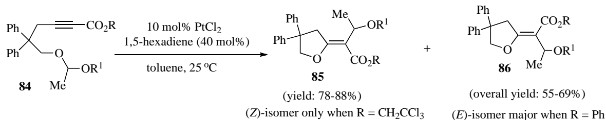
Scheme 27. Pt-Catalyzed stereoselective synthesis of dihydrofuran derivatives
