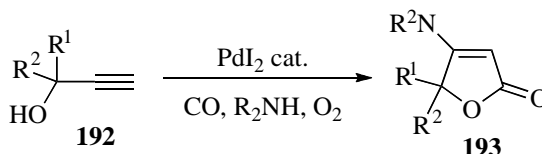
Scheme 60. PdI 2 -Catalyzed oxidative aminocarbonylation-cyclization
