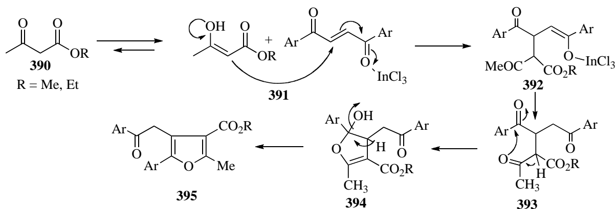
Scheme 115. \text{InCl}_3 -Catalyzed synthesis of tetrasubstituted furans
