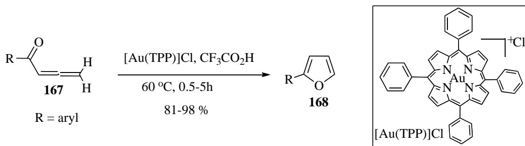
Scheme 52. Au(TPP)]Cl-Catalyzed cycloisomerization of allenones to furans
