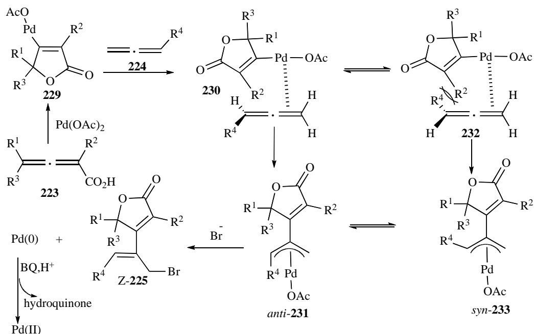
Scheme 72. Mechanism for the cross-coupling reactions
