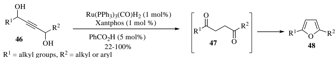
Scheme 15. Ru-Catalyzed isomerization of alkynediols to furans
