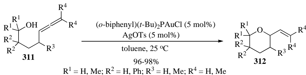
Scheme 93. Au-Catalyzed synthesis of pyrans under achiral conditions
