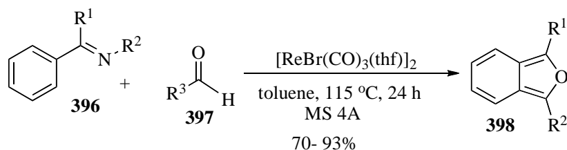
Scheme 116. Re-Catalyzed synthesis of isobenzofuran derivatives from aromatic ketimines
