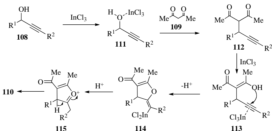
Scheme 35. Mechanism for the synthesis of tetrasubstituted furans
