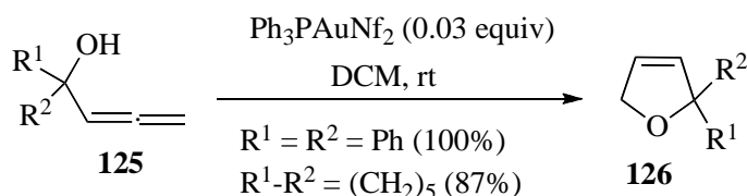
Scheme 39. Au-Catalyzed cyclization of \alpha -hydroxy allenes having a tert -OH
