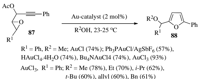
Scheme 28. Au-Catalyzed cycloisomerization of alkyloxiranes to furans
