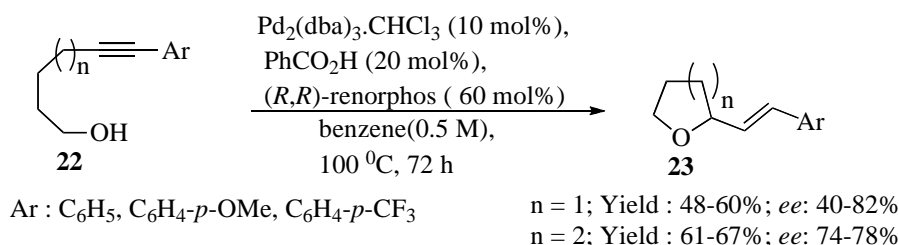
Scheme 7. Pd-Catalyzed hydroxylation of propargyl alcohols
