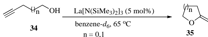
Scheme 11. La-Catalyzed hydroxylation of propargyl alcohols to furans
