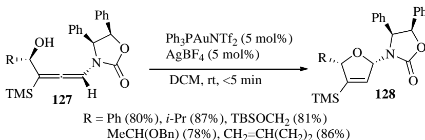
Scheme 40. Au-Catalyzed cycloisomerization of \alpha -hydroxyallene with chirality transfer
