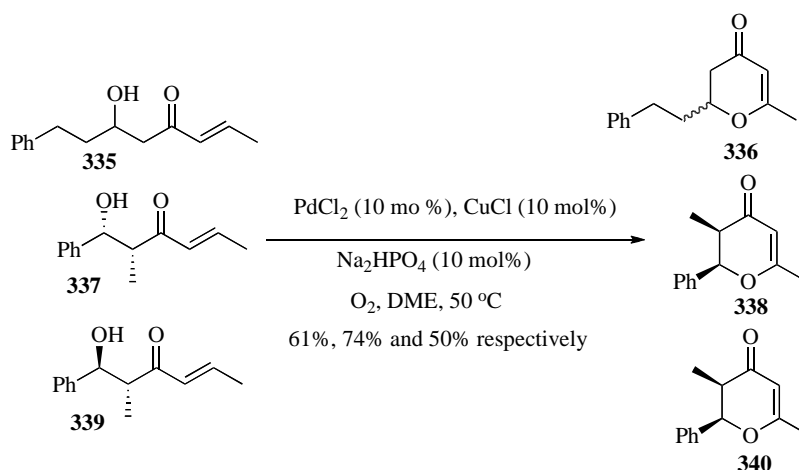
Scheme 100. Enantioselective synthesis of pyranones by Pd(II)-catalyzed reactions
