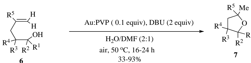
Scheme 4. Au-Catalyzed synthesis of tetrahydrofurans
