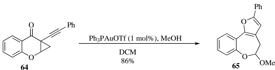
Scheme 21. Au-catalyzed synthesis of tricyclic furans
