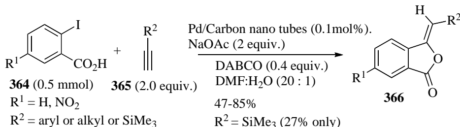
Scheme 108. Pd/carbon Nanotubes-Catalyzed synthesis of phthalides
