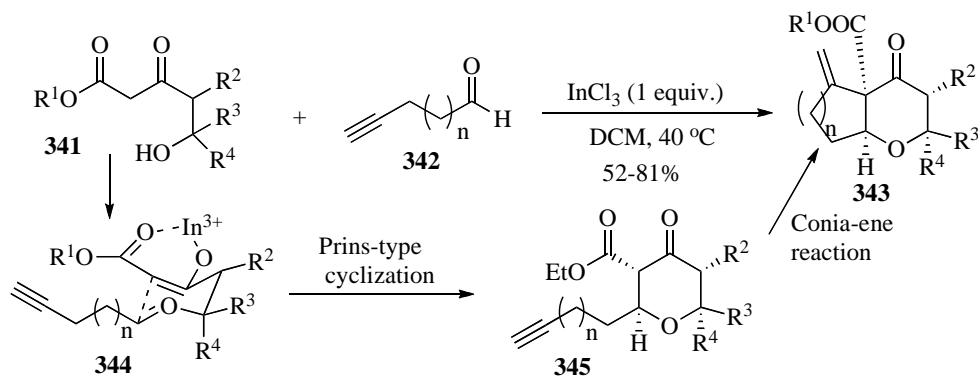
Scheme 101. In(III)-Mediated synthesis of highly functionalized 1-oxadecalins
