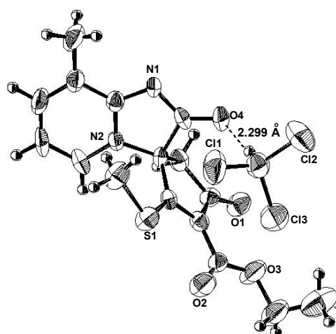
Figure 2. ORTEP drawing of 3b : \text{CHCl}_3
