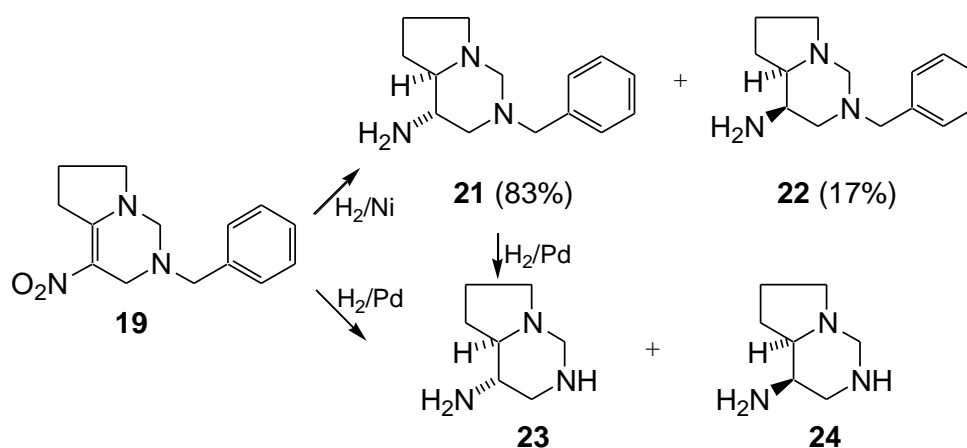
Scheme 4. Reduction of 19
