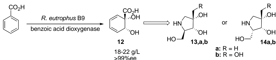
Figure 2. Design of hydroxylated piperidines and pyrrolidines from cis -dihydrodiols derived by enzymatic dihydroxylation
