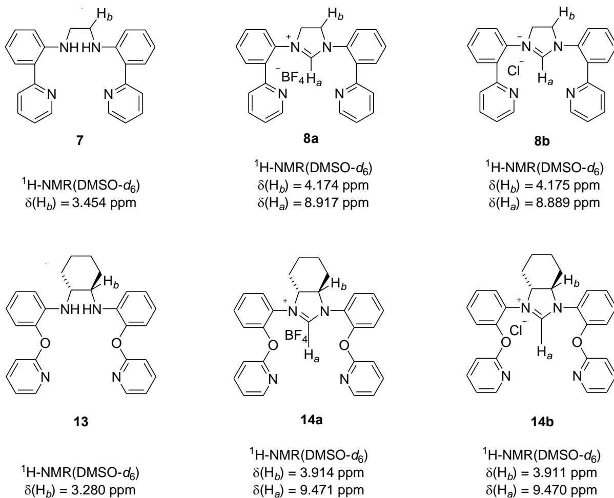
Figure 2. Selected chemical shifts [ \delta (ppm), downfield from tetramethylsilane] of diamines 7 and 13 , and imidazolinium salts 8 and 14
