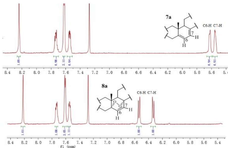
Figure 2. The partial 1 H NMR spectrums of compound 7a and 8a
