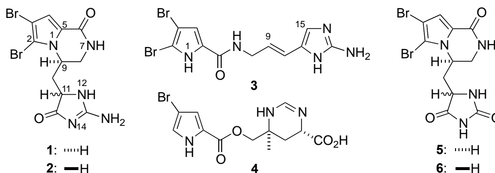
Figure 1. Structures of 1-6
