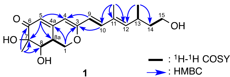
Figure 1. Selected 2D NMR correlations for isochromophilol A ( 1 )
