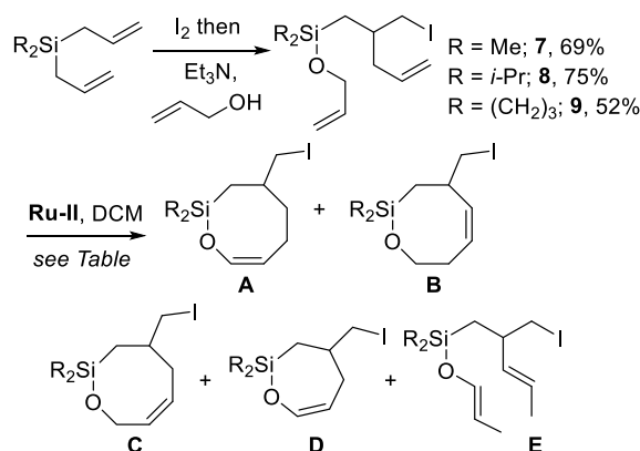
Scheme 4. Synthesis and RCM of differentially silicon-substituted dienes
