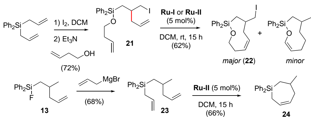
Scheme 8. RCM reactions of homoallyl ether 21 and non-ether 23
