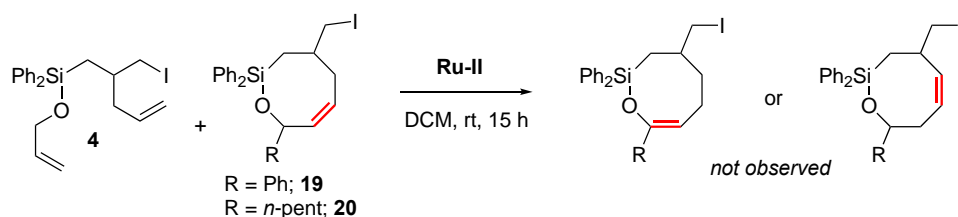
Scheme 7. RCM of 4 in the presence of 19 and 20
