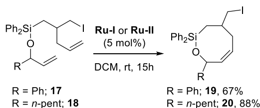
Scheme 6. Synthesis of phenyl and n -pentyl substituted oxasilacycles 19 and 20 by RCM
