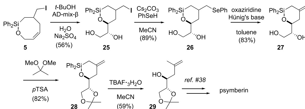
Scheme 12. Synthesis of compound 29 , a known synthetic precursor to the natural product psymberin, 38 from oxasilacycle 5
