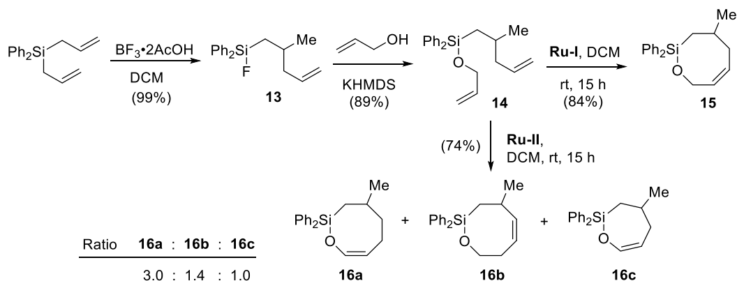
Scheme 5. Synthesis and RCM reactions of methyl-substituted dienyilsilane 14
