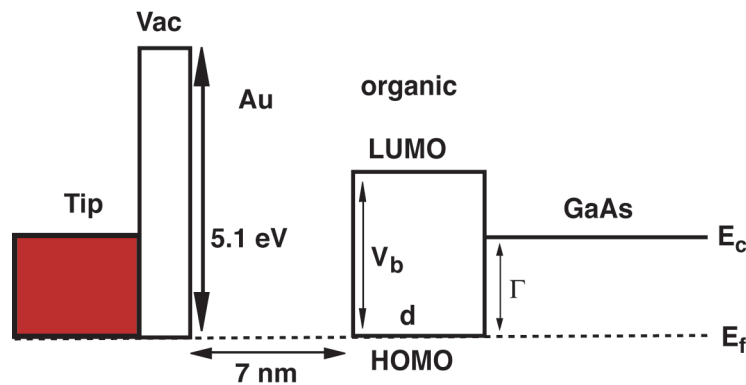
Figure 4. To calculate the transmission coefficient T_{hs} we have used three piecewise constant potentials for Au-organic-GaAs respectively, with the corresponding widths and heights, the height of the Au layer is zero because of the Fermi level alignment. HOMO and LUMO denotes highest occupied molecular orbital and lowest unoccupied molecular orbital respectively.
