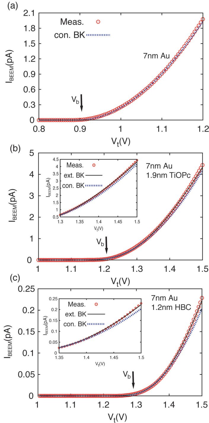
Figure 5. Averaged BEES spectra of Au/GaAs, Au/TiOPc/GaAs and Au/HBC/GaAs at 300 K. (a): Averaged BEES spectrum of 7 nm Au/GaAs, (b): 7 nm Au/1.9 nm TiOPc/GaAs and (c): 7 nm Au/1.2 nm HBC/GaAs. Solid lines are the calculated spectra using the extended Bell-Kaiser model, the dashed lines are calculated with the conventional Bell-Kaiser model, and the dots are the measured values. V_b denotes the Schottky barrier height.
