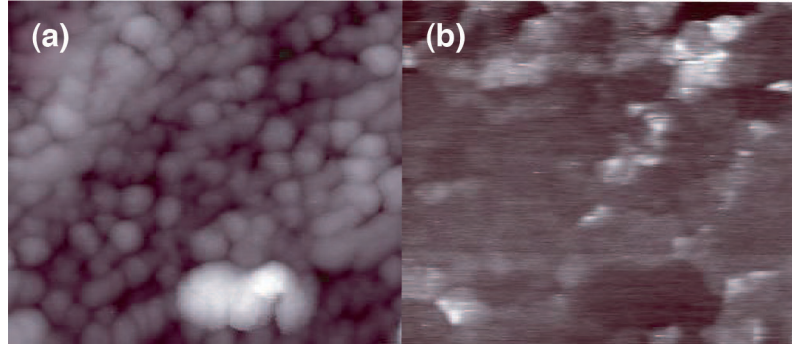
Figure 3. (a) STM topographic image of the Au/TiOPc/GaAs nanostructure. The image was recorded at T = 300 K, I_t = 5 nA, V_t = 1.4 V. The scansize is 200 \text{ nm} \times 200 \text{ nm} . (b) Corresponding BEEM image recorded simultaneously with the STM image. The color scale corresponds to 0, \dots, 1 pA, brighter areas indicate an enhanced electron transmission.
