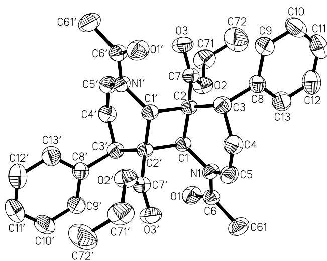
Figure 1. ORTEP drawing of anti dimer ( 2a ) (Displacement ellipsoids at 50% probability level).
