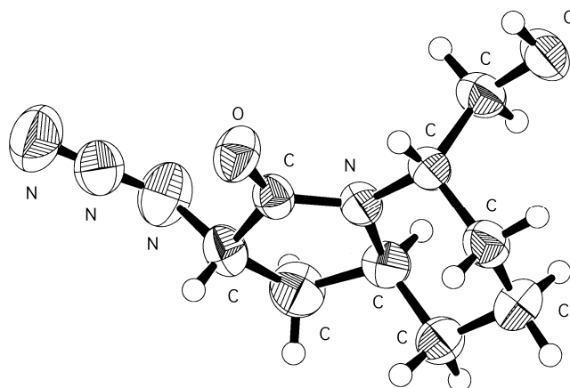
Figure 2. ORTEP diagram of 20
