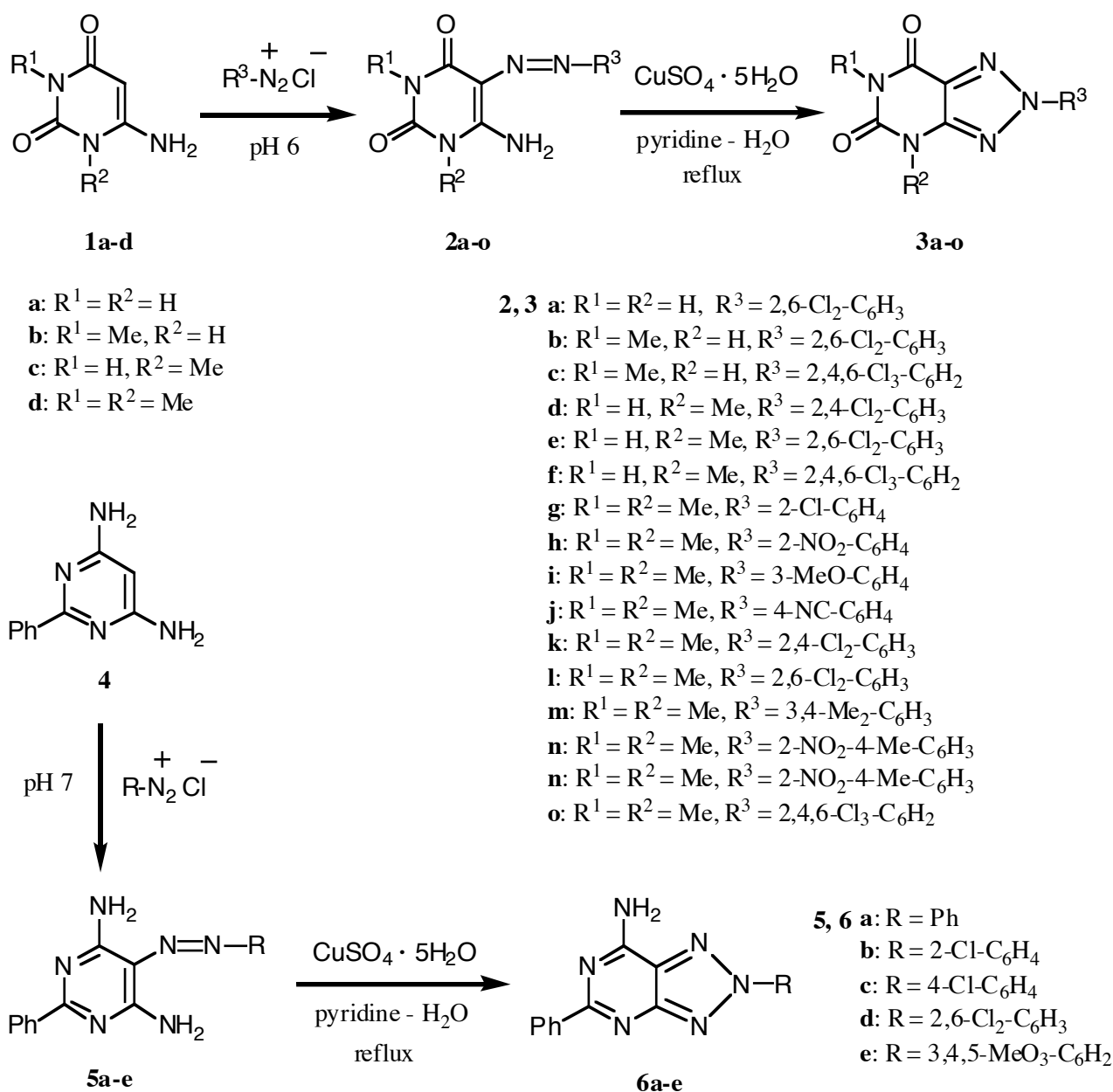
Scheme 1
