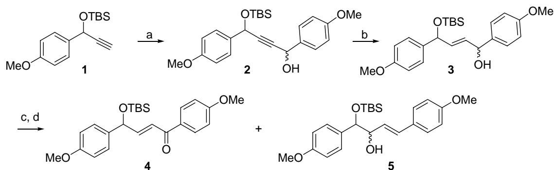
Scheme 2 Reagents and Conditions: (a) n -BuLi, HMPA, p -anisaldehyde, THF, -78 °C, 90%; (b) Red-Al ® , THF, 0 °C to rt, 66%; (c) column chromatography on silica gel; (d) MnO 2 , CH 2 Cl 2 , ultrasound, rt, 38% of 4 and 11% of 5 each from 3 .
