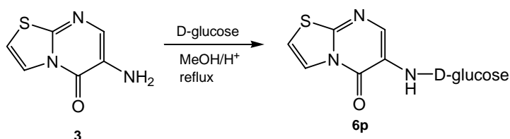
Scheme 3. Preparation of the glycosides 6a-p
