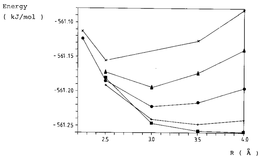
Figure 14 : Sections through the energy hypersurface for the Meth-OM-DHN/ CH_2O supermolecule. Rehybridisation factors : 0.0 ( ■ ), 0.1 ( + ), 0.2 ( ● ), 0.3 ( ▲ ) and 0.4 ( × ).
