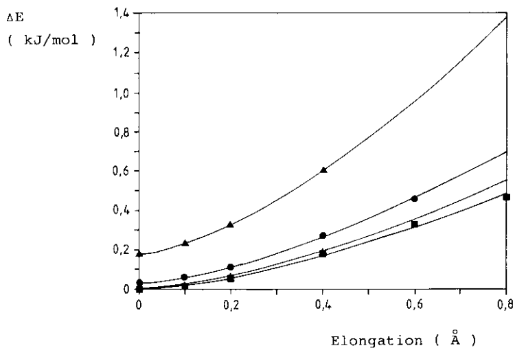
Figure 10 : Influence of elongation on approach energy \Delta E (cfr. Figure 4). (■) : R = , (+) : R = 3.5 \text{ \AA} , (●) : R = 3.0 \text{ \AA} and (▲) : R = 2.5 \text{ \AA} .
