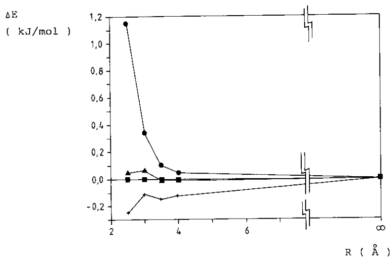
Figure 7 : Influence of methyl substitution on the energy gain due to the approach of the formaldehyde molecule, relative to Meth-OM-DHN ( \Delta E ). (■) = 0M, (+) = 2M, (●) = 5M and (▲) = 6M.
