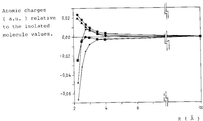
Figure 6 : Influence of the intermolecular approach on the atomic charge of the formaldehyde molecule relative to the values for the isolated molecules. ( ■ ) = C 25 , ( + ) = O 26 , ( ● ) = H 27 , ( ▲ ) = H 28 , ( × ) = total for the CH 2 O molecule.
