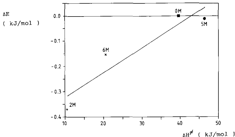
Figure 12 : Correlation of the elongation energy \Delta E_{el} and activation enthalpy \Delta H^\ddagger for an intermolecular distance R of 3.5 \text{ \AA} for the methyl substituted analogues.
