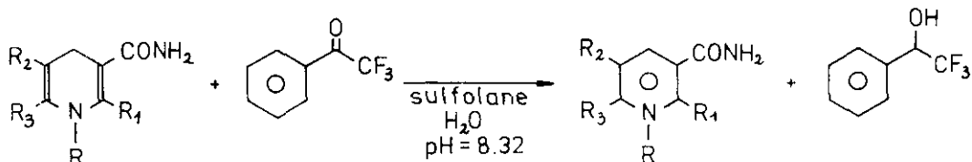
Figure 2 : The reaction between the dihydronicotinamides and trifluoroacetophenone.
