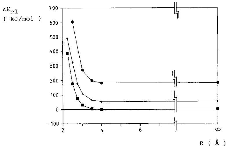
Figure 9 : Influence of the intermolecular approach on the elongation energy \Delta E_{e1} for elongation values of 0 \text{ \AA} (■), 0.2 \text{ \AA} (+) and 0.4 \text{ \AA} (●). The elongation energy \Delta E_{e1} is defined as the energy difference between a geometry with a dihydronicotinamide molecule which has an elongated CH bond and a geometry with its equilibrium geometry.
