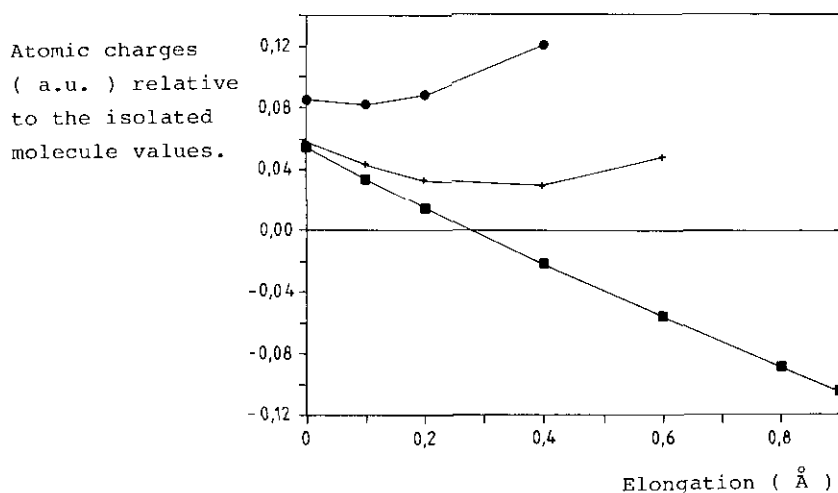
Figure 11 : Evolution of the net atomic charge for the H 2 atom upon elongation for various intermolecular distances. ( ■ ) : R = ∞, ( + ) : R = 3.0 Å and ( ● ) : R = 2.5 Å.
