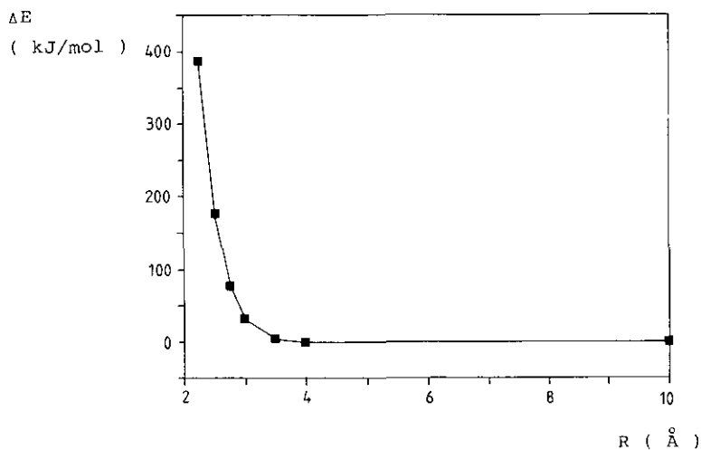
Figure 4 : Influence of the approach of the formaldehyde molecule on the energy of the supermolecule, relative to the isolated molecules ( \Delta E ).
