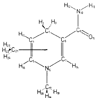
Figure 1 : Nomenclature conventions and atom numbering for the methyl substituted N -methyl-1,4-dihydronicotinamides.
