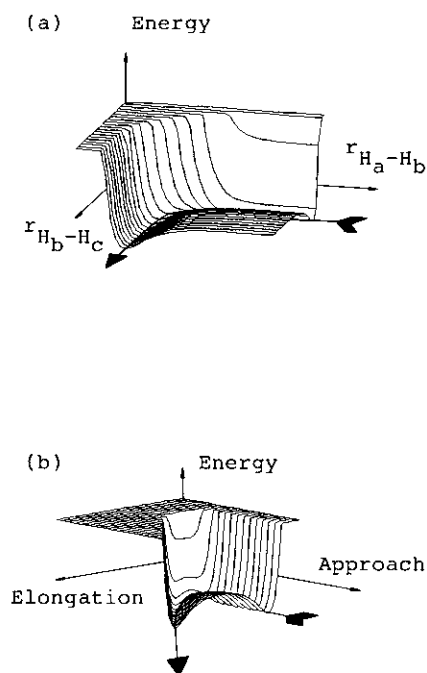
Figure 8a and b. : Energy hypersurface for a collinear attack of a hydride ion H_a^- on a hydrogen molecule H_b-H_c (a) using the H_aH_b and H_bH_c distances as variables and (b) using variables describing elongation ( r_{H_a-H_b} - r_{H_a-H_b}, 0 ) and approach ( r_{H_a-H_c} ).
