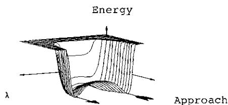
Figure 13 : Energy hypersurface for a S_N2 type reaction such as the collinear attack of a hydride ion H_a^- on a hydrogen molecule H_b-H_c in terms of approach A_p and rehybridisation factor \lambda ( see text ).
