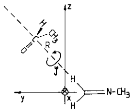
Figure 3 : Geometrical parameters describing the approach of acetaldehyde towards the dihydropyridinamides.
