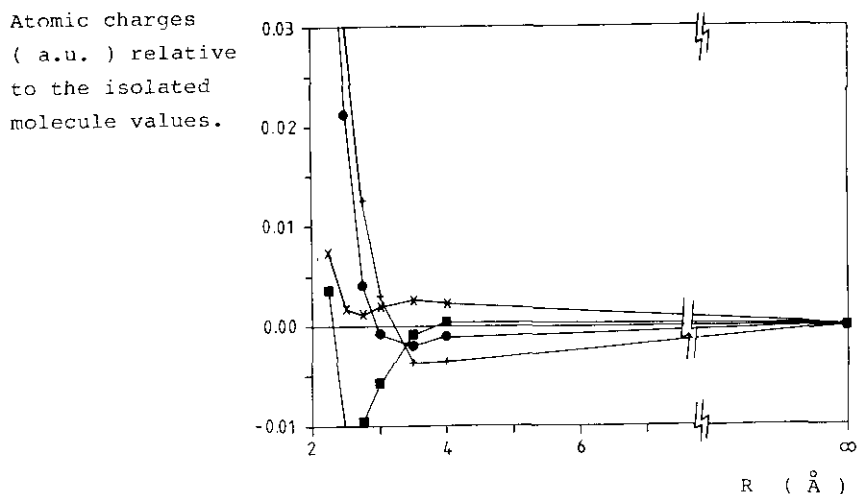
Figure 5 : Influence of the intermolecular approach on the atomic charge of the methylene group relative to the values for the isolated molecules. ( + ) = H 2 , ( × ) = H 3 , ( ■ ) = C 1 and ( ● ) = total for the CH 2 group.
