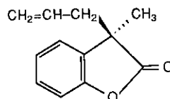
(R)-(+)- \underline{5}
