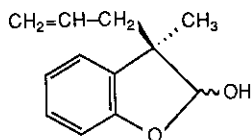
(R)- \underline{4}
