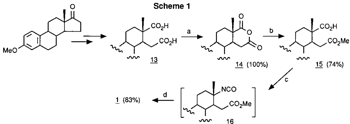
Scheme 1
