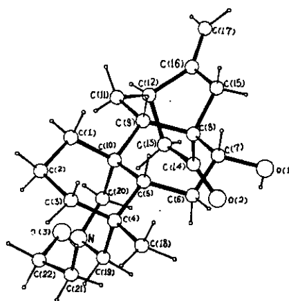
Fig. 2 Crystal structure of 3, showing the atom-labeling scheme
