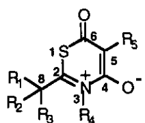
1a ; (R 1 , R 2 , R 3 = alkyl)
