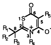
1b ; (R 1 , R 2 , or R 3 = H)
