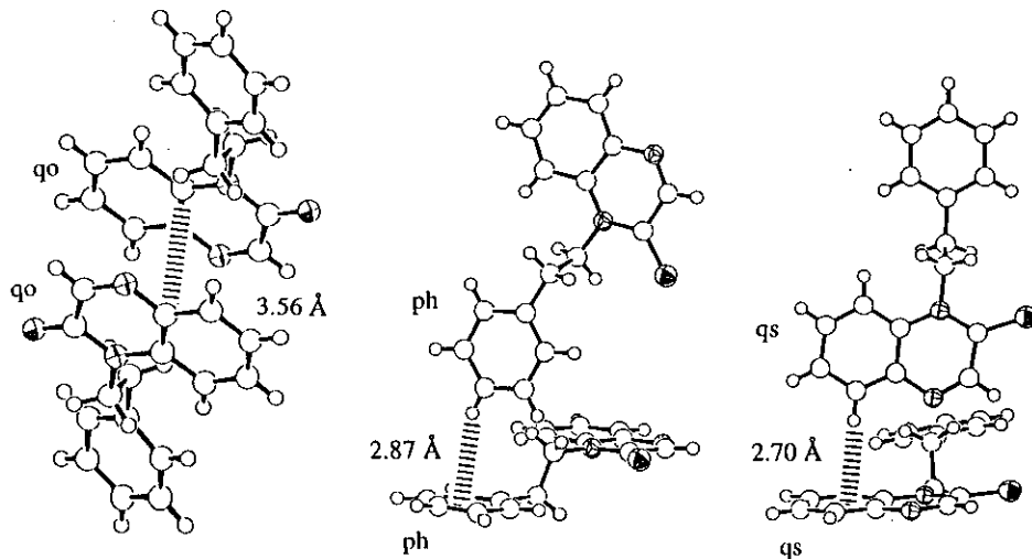
Figure 4 Views of aromatic interactions for 2a (left) and 4a (center and right)
