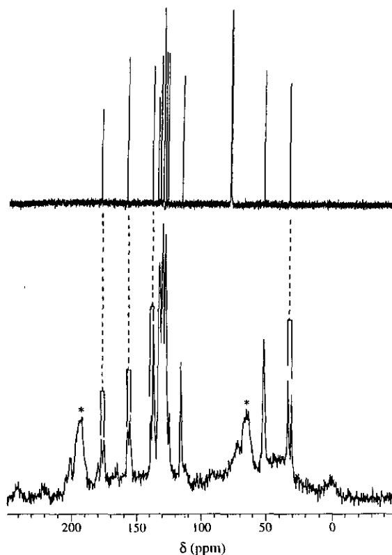
Figure 1 ^{13}\text{C} Nmr spectra of 4a ; (top) in \text{CDCl}_3 solution, (bottom) in the crystalline state by CPMAS mode ; spinning side band (*)
