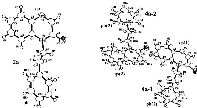
Figure 2 ORTEP drawings of 2a (left) and 4a (right) showing 50 and 40% probability displacement ellipsoids
