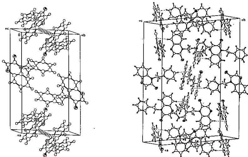
Figure 3 Packing diagrams of molecules in the unit cells of 2a (left) and 4a (right)
