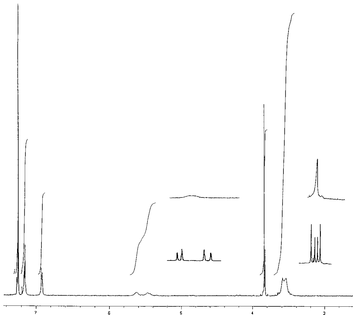
Figure 4. 1 H NMR Spectrum of 3d in CDCl 3 (500 MHz) with signals measured at -10 °C (below) and at 50 °C (above).
